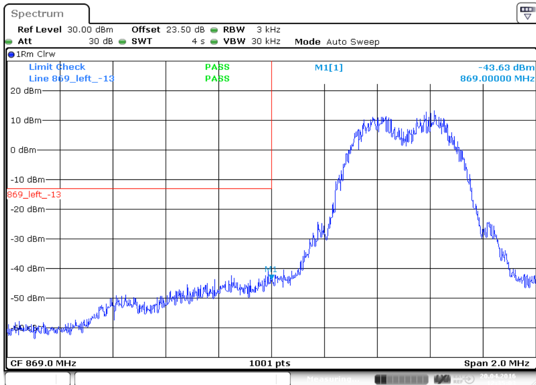
plot 8.3.1.1-#1 Intermodulation: §22.917, §2.1051; Test results; Downlink; GSM Lower Band Edge
