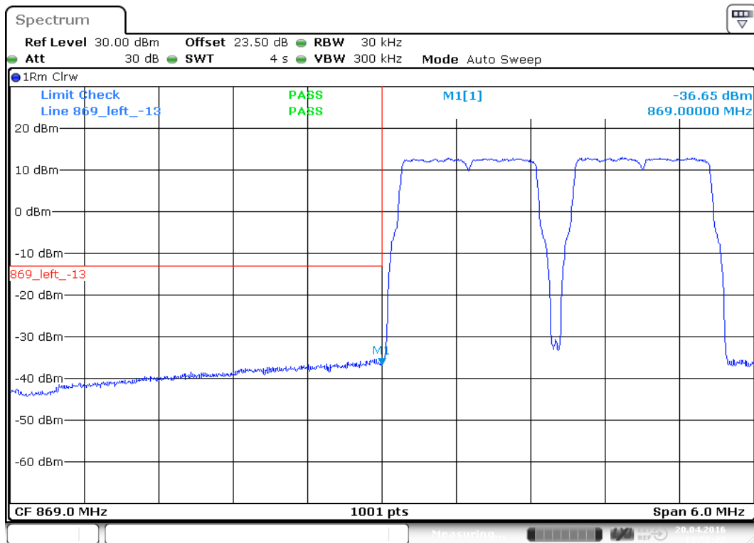
plot 8.3.1.5-#1 Intermodulation: §22.917, §2.1051; Test results; Downlink; LTE Lower Band Edge
