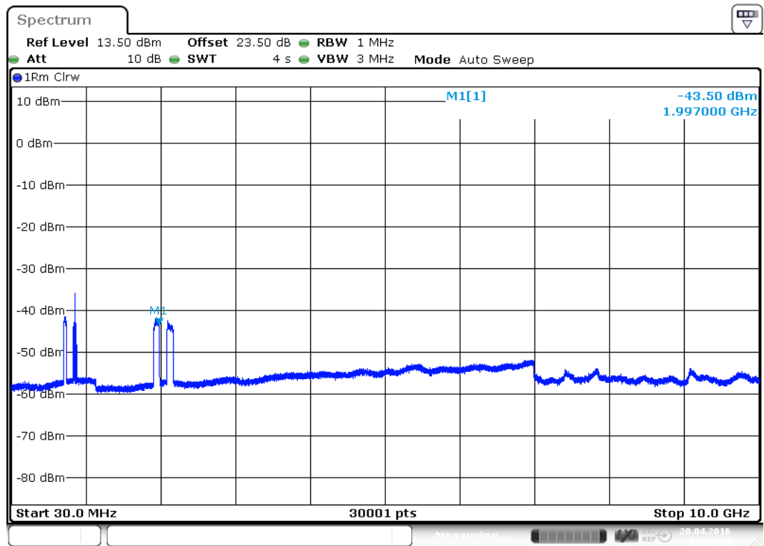
plot 7.3.1.3-#1 Spurious Emissions at Antenna Terminals: §22.917, §2.1051; Test results; Downlink; CDMA; carrier (881,5MHz) notched
