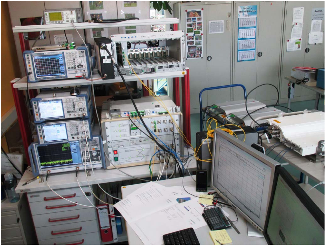
Measurement Equipment
