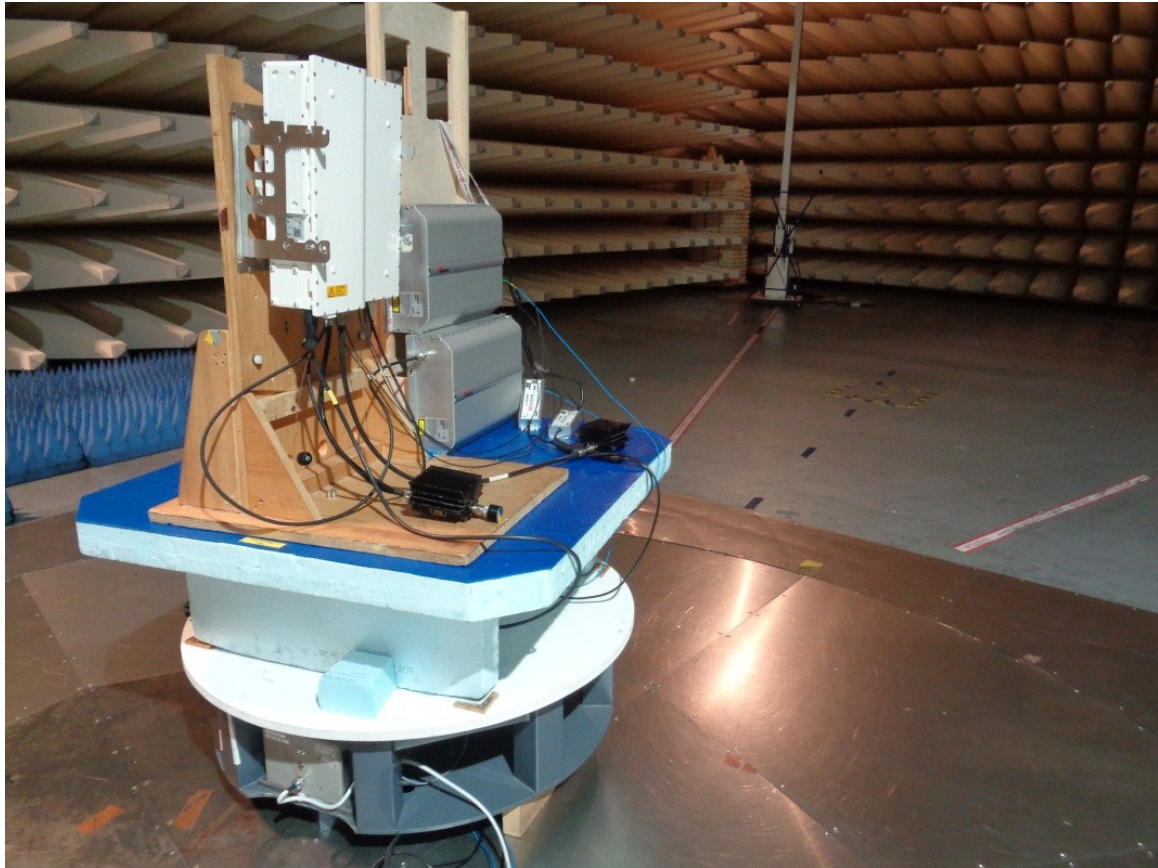
Test setup: Field Strength Emission
