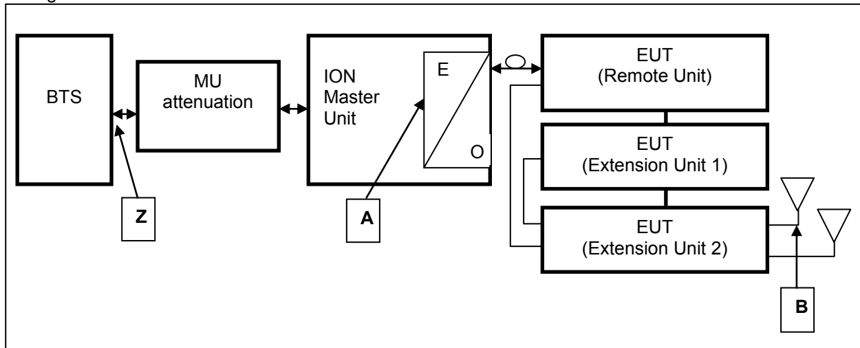
figure 2.1.4-#1 Block diagram of measurement reference points
