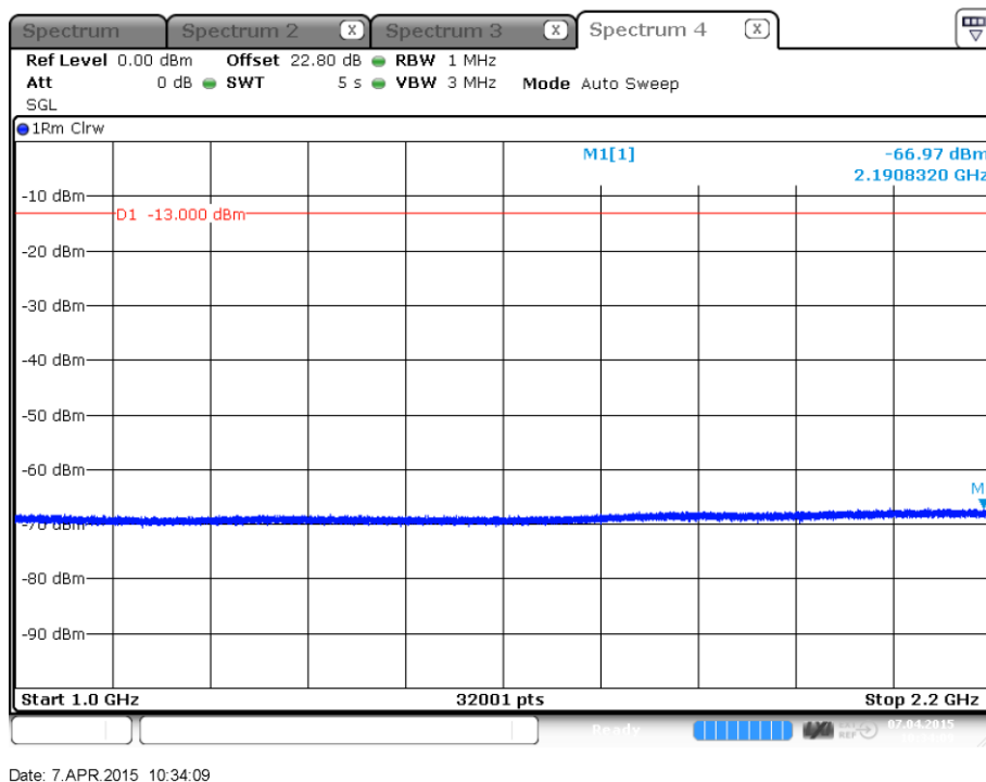
plot 7.3.1.2-#2 Spurious Emissions at Antenna Terminals: §27.53, §2.1051; Test results; Downlink; LTE; 10 MHz signal; 1 GHz – 2.2 GHz; carrier notched
