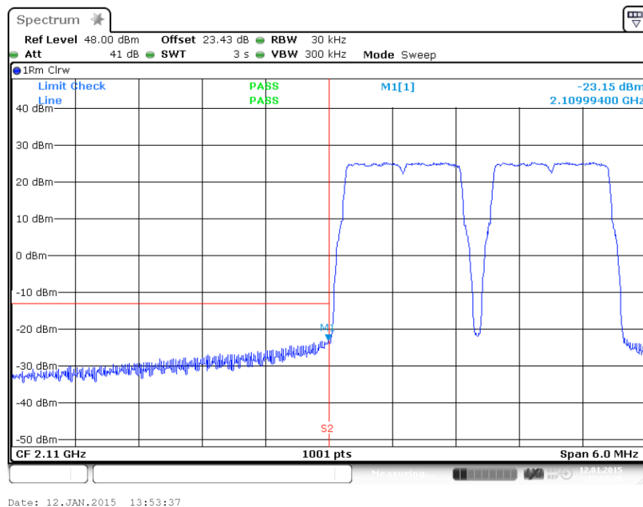
plot 8.3.1.3-#1 Intermodulation: $27.53, $2.1051; Test results; Downlink; LTE Lower Band Edge
