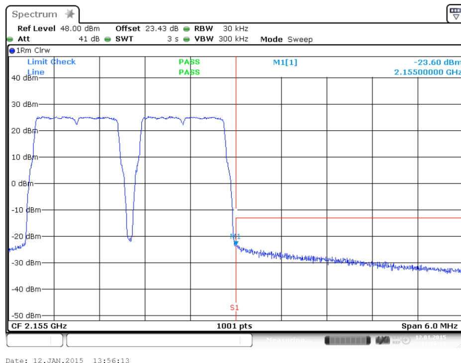
plot 8.3.1.3-#2 Intermodulation: $27.53, $2.1051; Test results; Downlink; LTE Upper Band Edge
