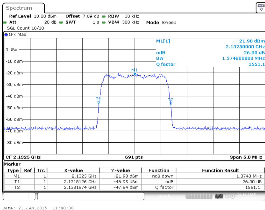
plot 6.3.2.1-#2 Occupied Bandwidth: $2.1049; Test results; 26dB Bandwidth; CDMA Input
