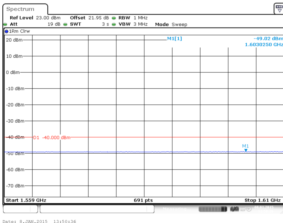
plot 7.3.1.3-#1 Spurious Emissions at Antenna Terminals: §27.53, §2.1051; Test results; Downlink; Measurement in the band of 1559 MHz – 1610 MHz acc. to 27.53(f)
