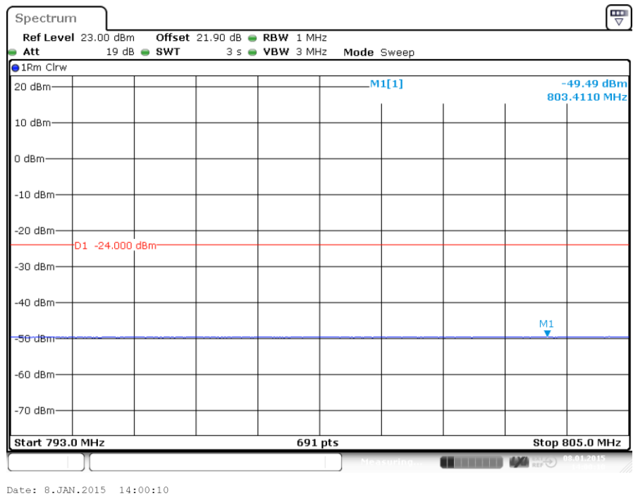
plot 7.3.1.1-#3 Spurious Emissions at Antenna Terminals: §27.53, §2.1051; Test results; Downlink; LTE 728 – 746MHz; 793 MHz – 805 MHz
