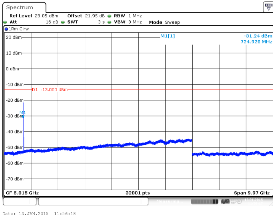
plot 7.3.1.2-#1 Spurious Emissions at Antenna Terminals: §27.53, §2.1051; Test results; Downlink; LTE 746 – 757MHz; 30 MHz – 10 GHz; carrier (751,5MHz) notched
