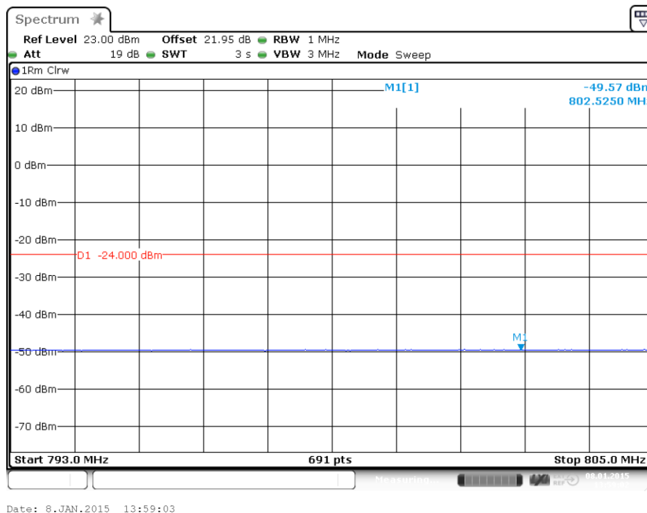
plot 7.3.1.2-#3 Spurious Emissions at Antenna Terminals: §27.53, §2.1051; Test results; Downlink; LTE 746 – 757MHz; 793 MHz – 805 MHz
