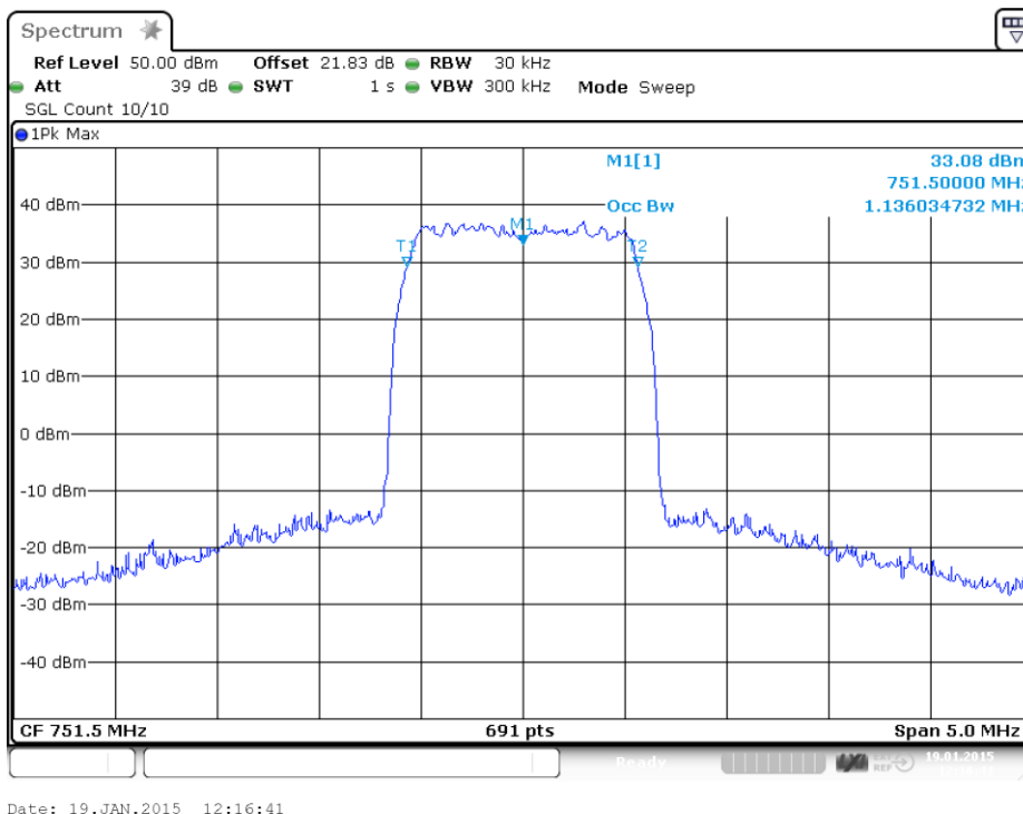
plot 6.3.1.2-#1 Occupied Bandwidth: $2.1049; Test results; Downlink; LTE 746 – 757MHz Output
