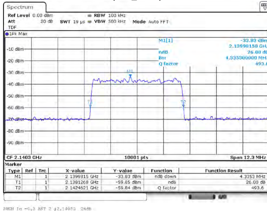
Input Signal
