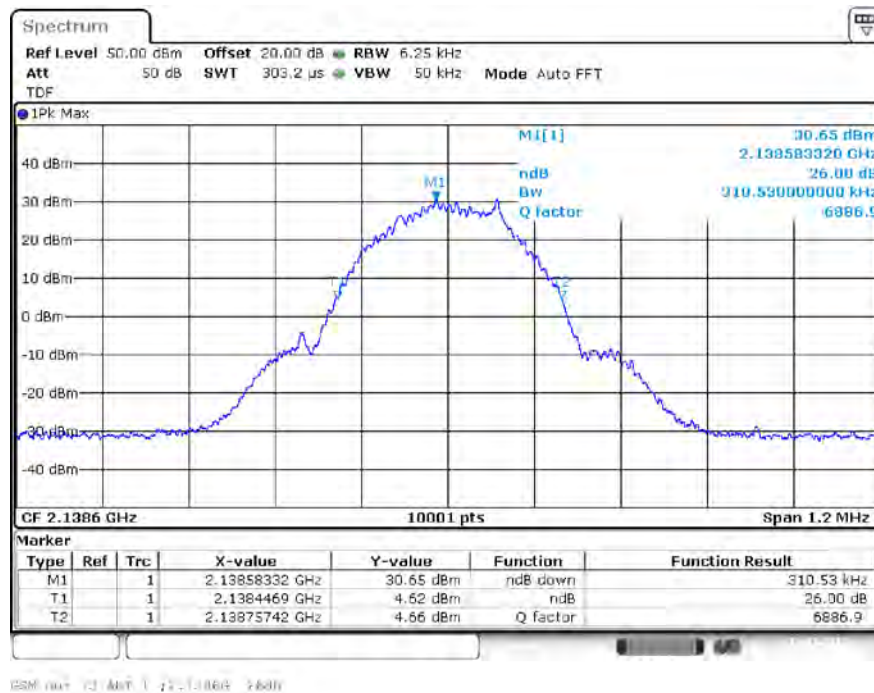
Output Signal
