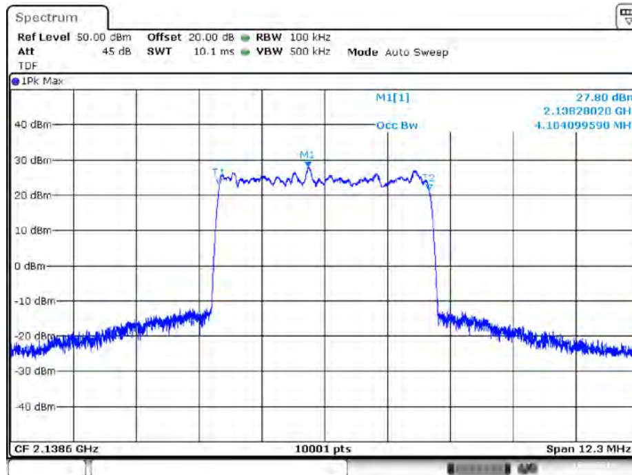
Output Signal
