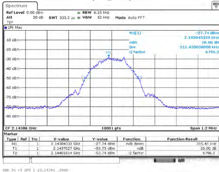
Input Signal
