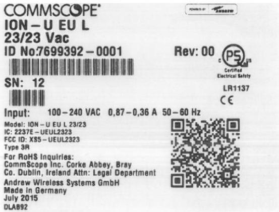
picture 8.1: label EUT
