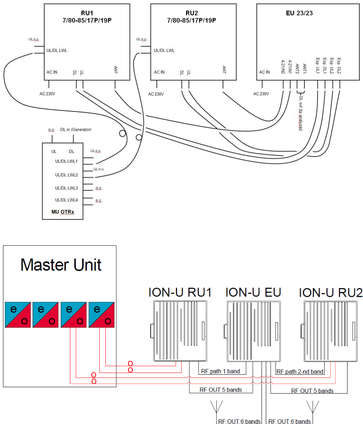
picture 8.3: Test configuration
