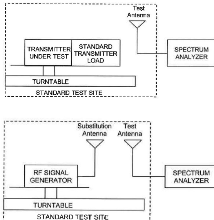
Figure #8.3 Substitution methods TIA/EIA-603-C
