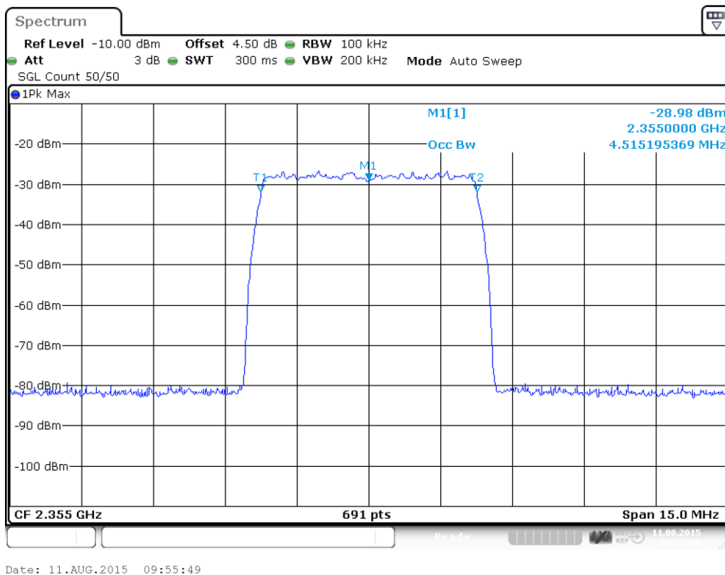
plot 6.3.1.1-#2 Occupied Bandwidth: $2.1049; Test results; Downlink; LTE; 5 MHz signal; OBW 99% Input
