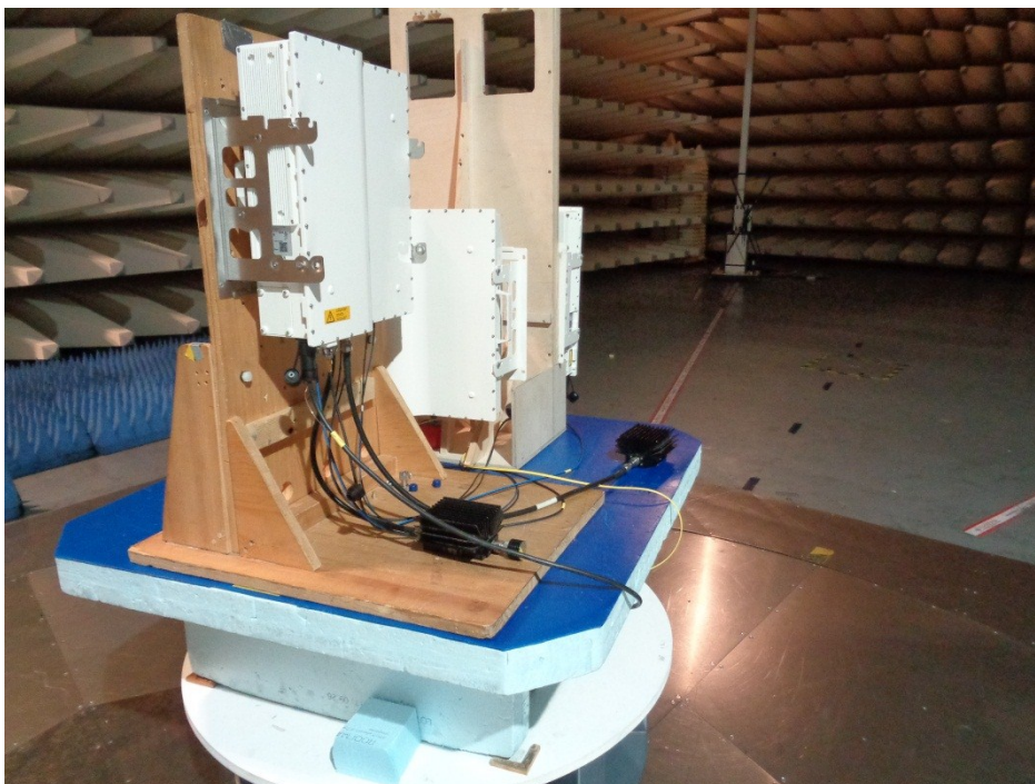
picture 8.3: Test setup
