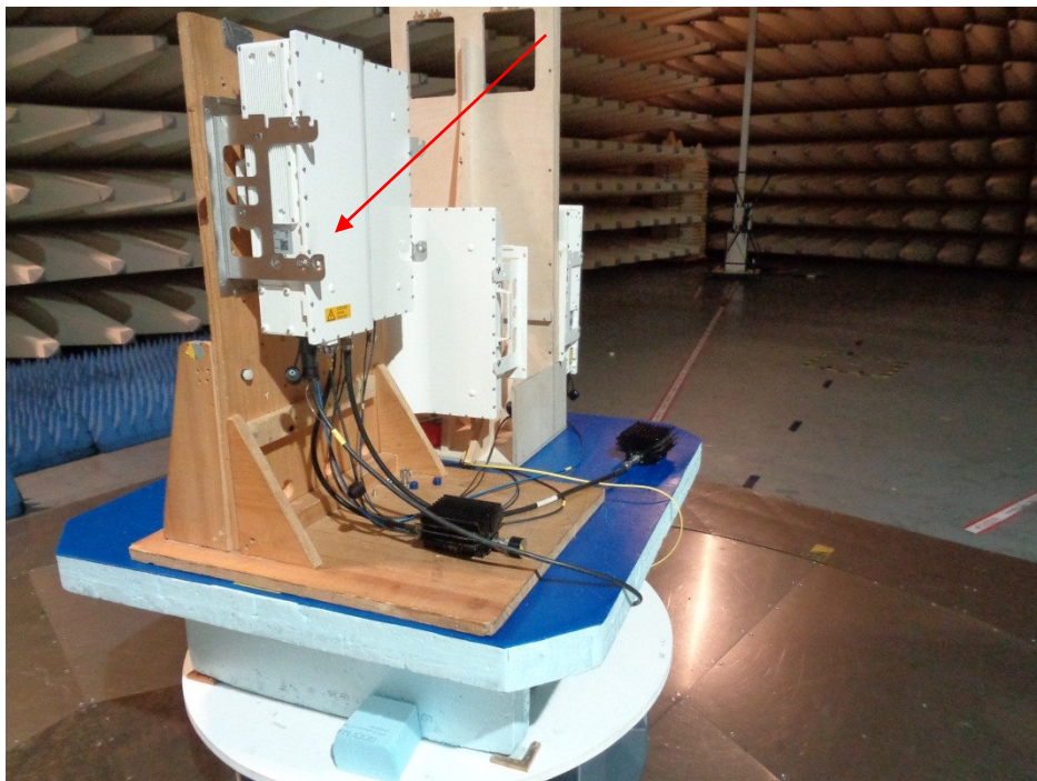
Test setup: Field Strength Emission
