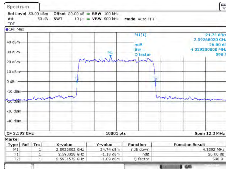
Output Signal
