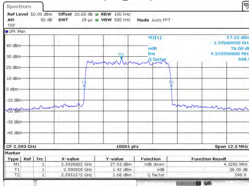
Input Signal
