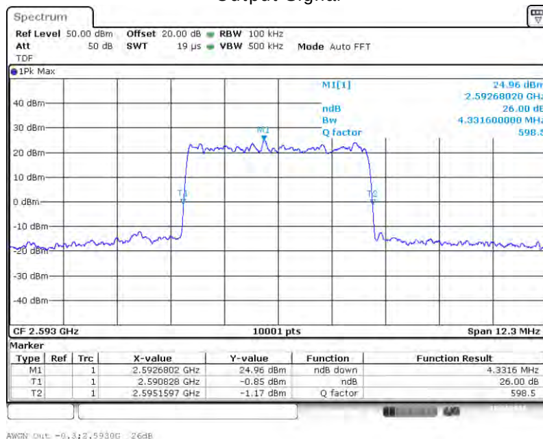
Output Signal
