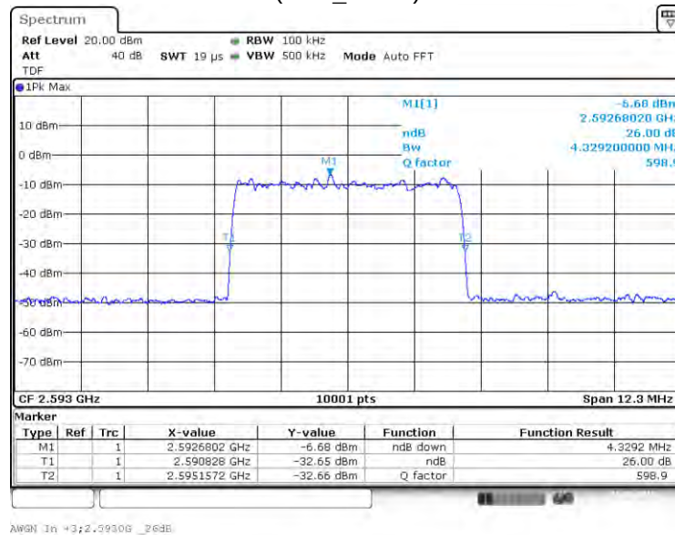
Input Signal
