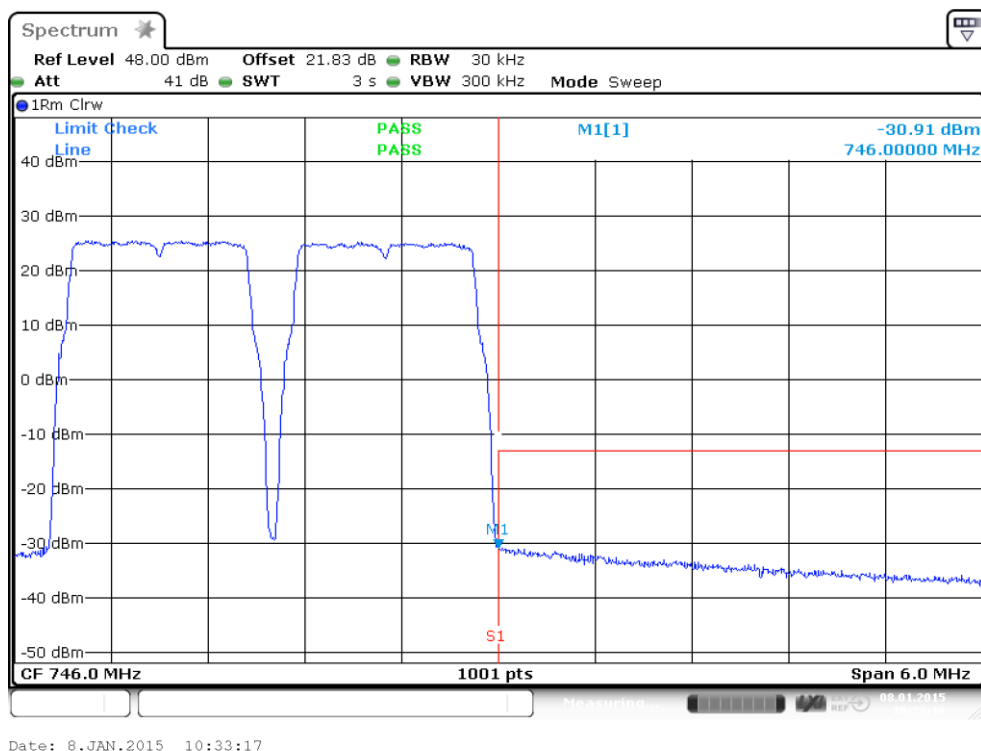
plot 8.3.1.1-#2 Intermodulation: $27.53, $2.1051; Test results; Downlink; LTE 728 – 746MHz Upper Band Edge
