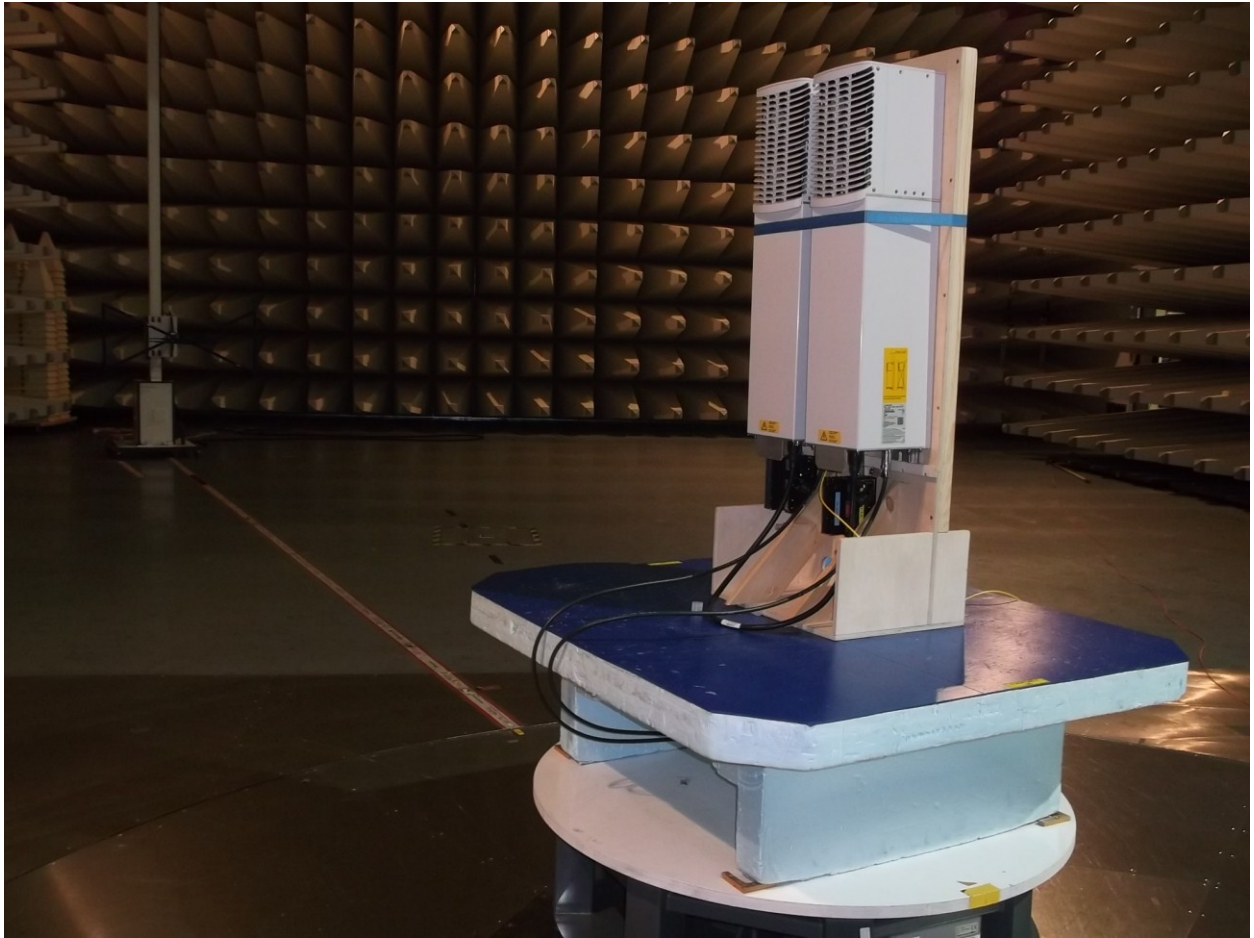
picture 1: Test setup: Field Strength Emission <1 GHz @10m in the SAC
