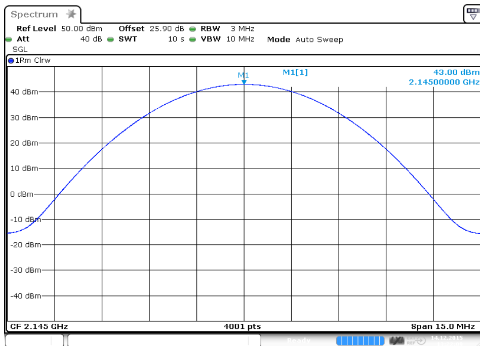
plot 5.3.1.1-#1 RF Power Out: §27.50, §2.1046; Test results; Downlink; CDMA Middle
