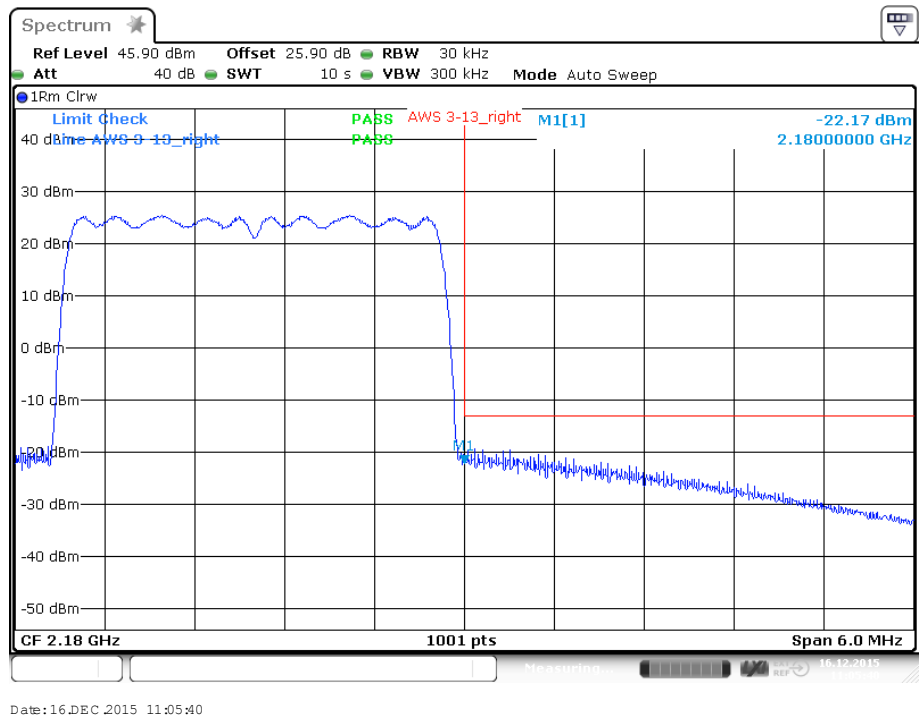
plot 8.3.1.1-#2 Intermodulation: §27.53, §2.1051; Test results; Downlink; CDMA Upper Band Edge
