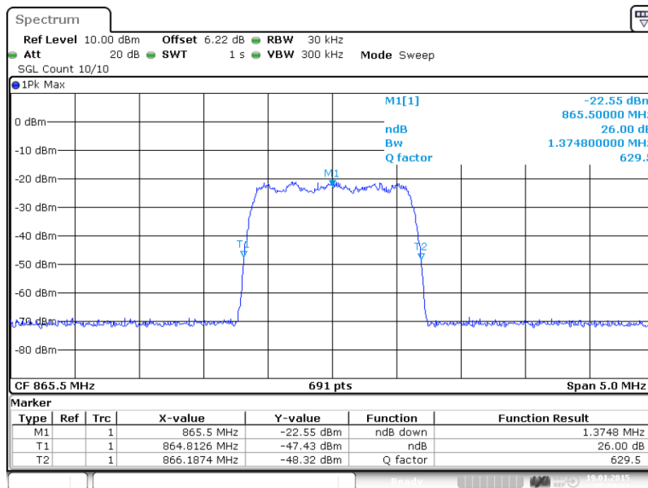
plot 6.3.2.3-#2 Occupied Bandwidth: §90.210, §2.1049; Test results; 26dB Bandwidth; CDMA Input
