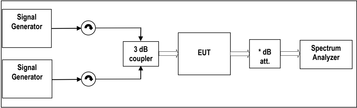
External Attenuator DL x dB = 20 dB figure 8-#1 Test setup: Intermodulation: §90.691, §2.1051
