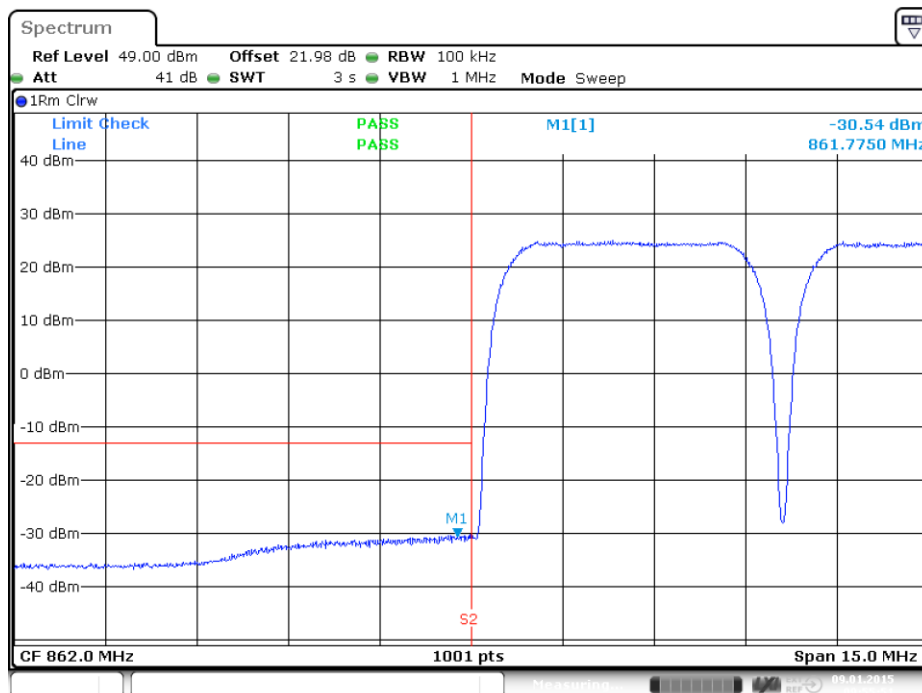
plot 8.3.1.4-#1 Intermodulation: §90.691, §2.1051; Test results; Downlink; WCDMA Lower Band Edge
