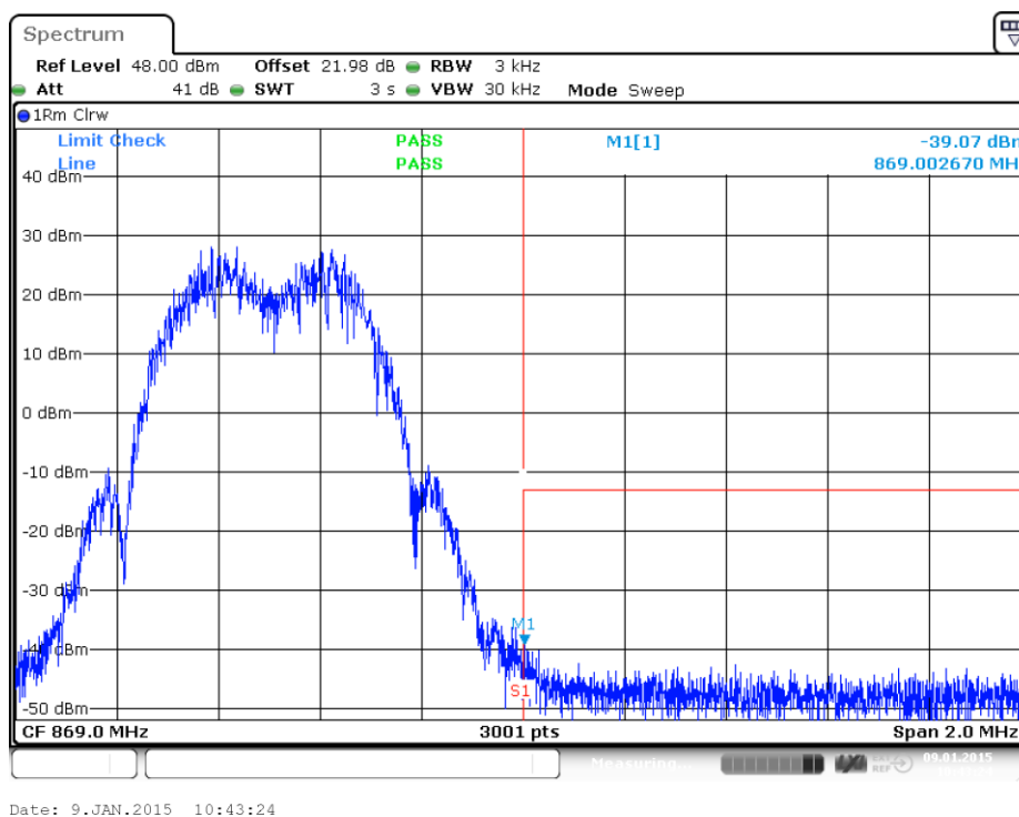
plot 8.3.1.2-#2 Intermodulation: §90.691, §2.1051; Test results; Downlink; EDGE Upper Band Edge
