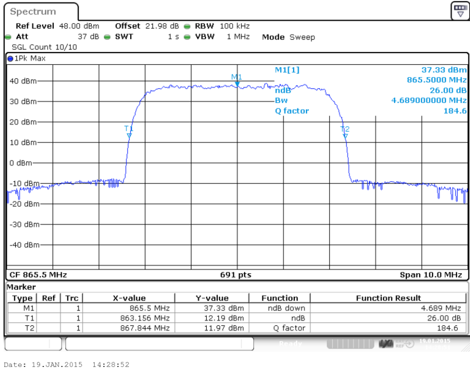
plot 6.3.2.4-#1 Occupied Bandwidth: $90.210, $2.1049; Test results; 26dB Bandwidth; WCDMA Output
