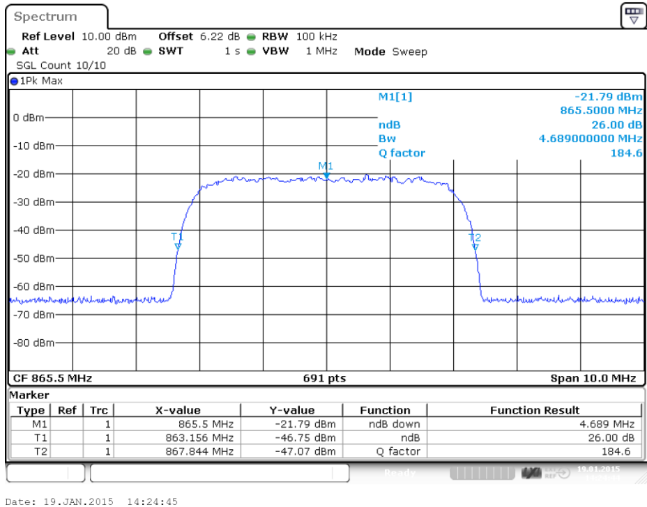
plot 6.3.2.4-#2 Occupied Bandwidth: $90.210, $2.1049; Test results; 26dB Bandwidth; WCDMA Input
