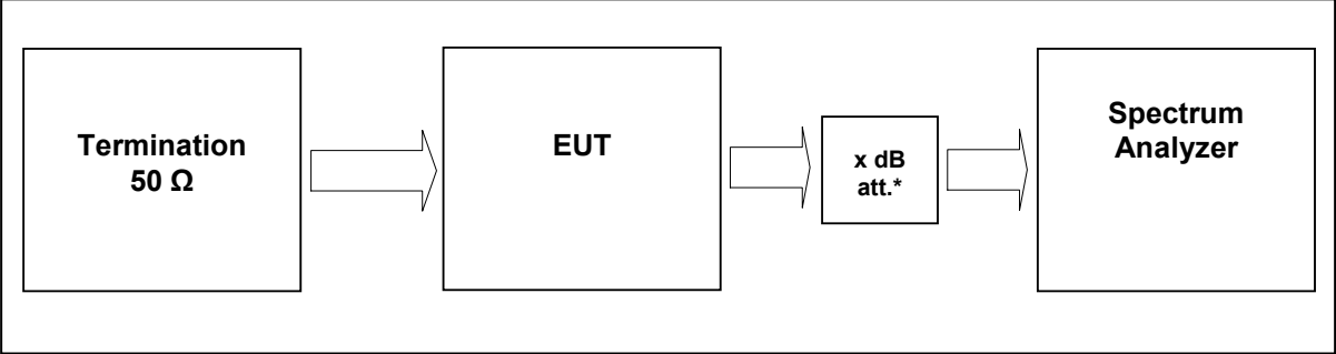
External Attenuator DL x dB = 20 dB figure 11-#1 Test setup: Noise
