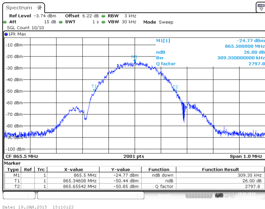
plot 6.3.2.2-#2 Occupied Bandwidth: $90.210, $2.1049; Test results; 26dB Bandwidth; EDGE Input
