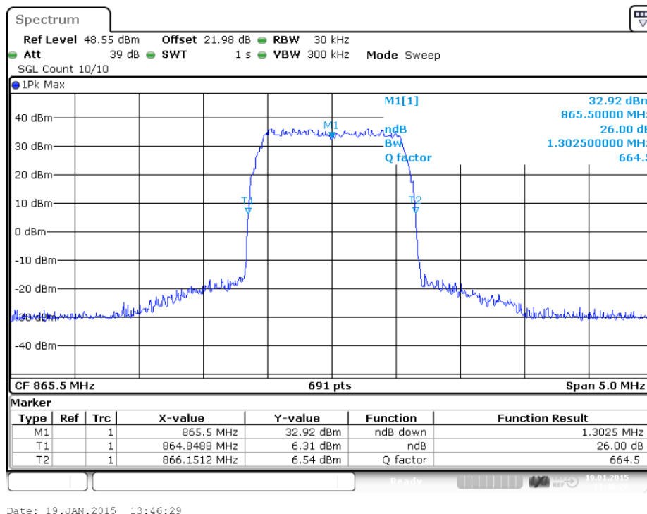
plot 6.3.2.5-#1 Occupied Bandwidth: $90.210, $2.1049; Test results; 26dB Bandwidth; LTE Output
