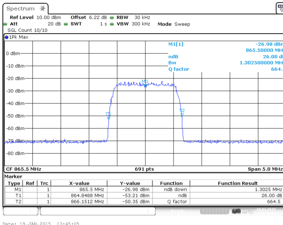
plot 6.3.2.5-#2 Occupied Bandwidth: $90.210, $2.1049; Test results; 26dB Bandwidth; LTE Input
