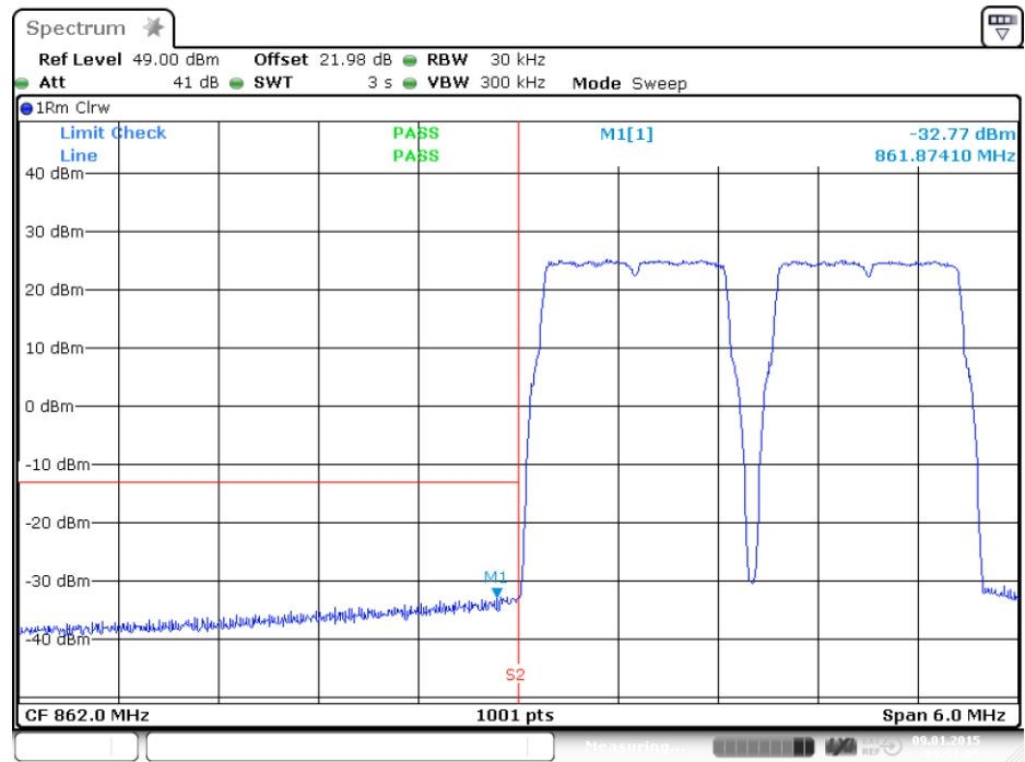
plot 8.3.1.5-#1 Intermodulation: §90.691, §2.1051; Test results; Downlink; LTE Lower Band Edge
