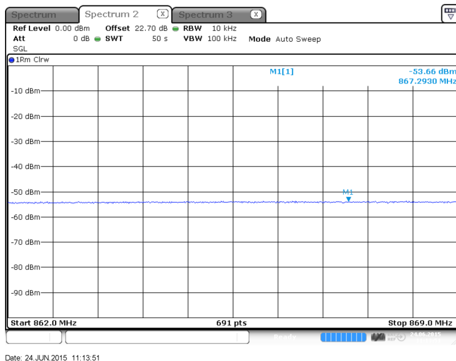
plot 11.3.1-#1 Noise; Test results; Downlink;
