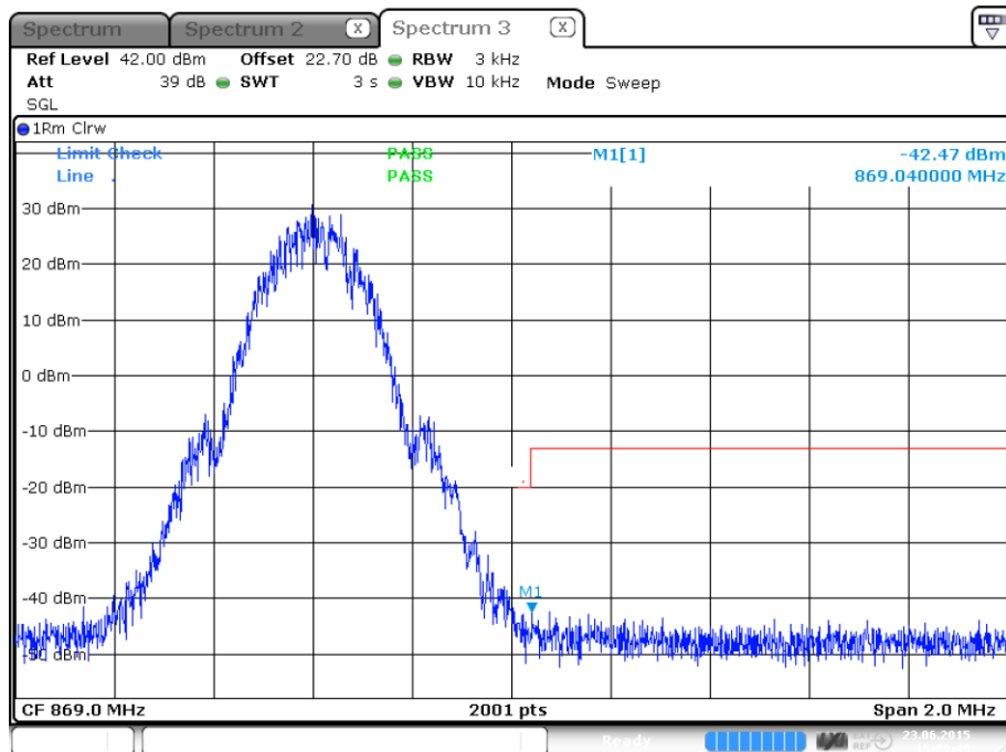
plot 9.3.1.1-#2 Emission Mask: §90.691, §2.1051; Test results; Downlink; GSM < 1MHz to band edge Upper Band Edge
