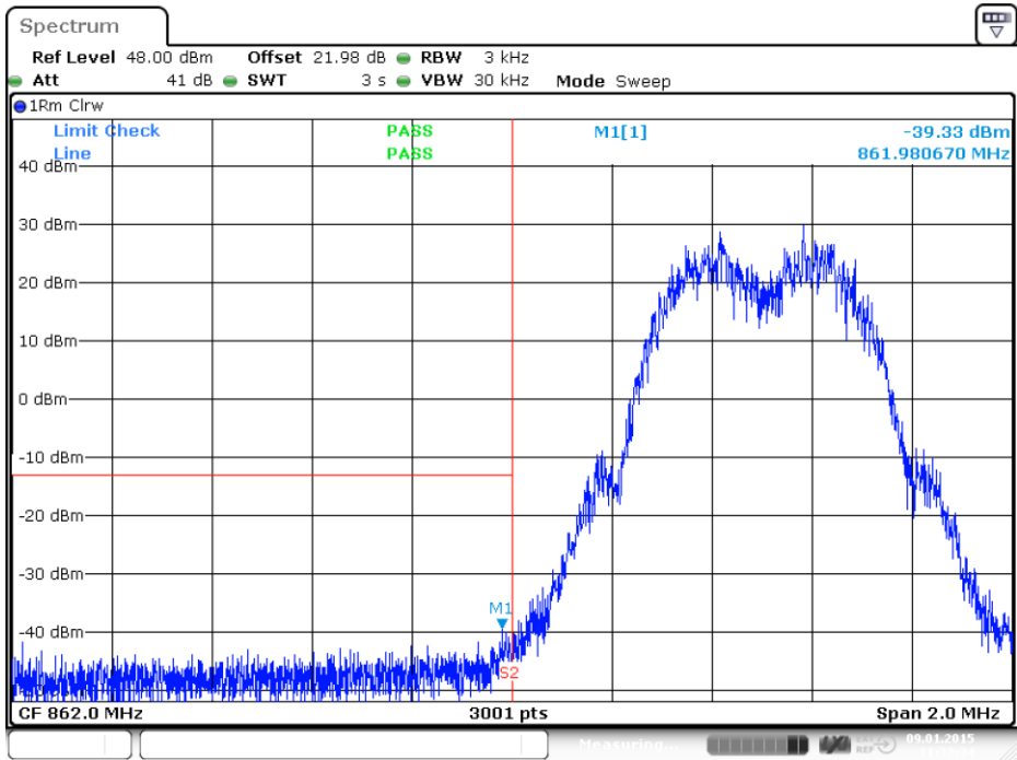
plot 8.3.1.1-#1 Intermodulation: §90.691, §2.1051; Test results; Downlink; GSM Lower Band Edge
