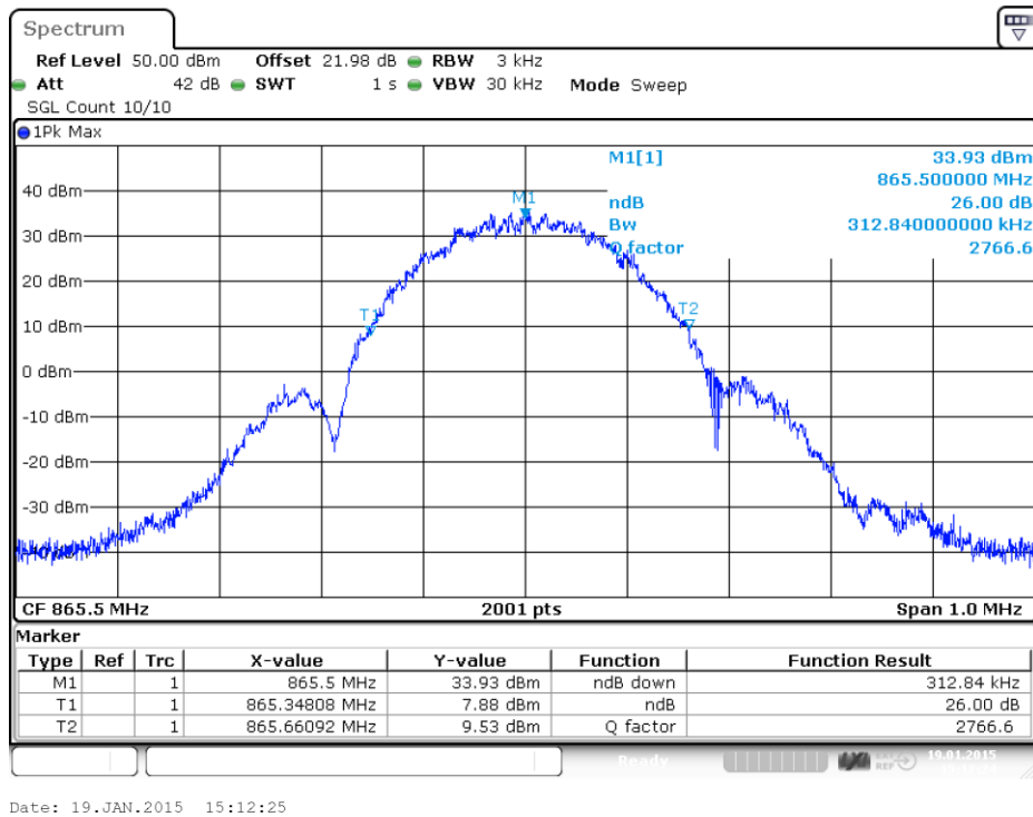
plot 6.3.2.2-#1 Occupied Bandwidth: $90.210, $2.1049; Test results; 26dB Bandwidth; EDGE Output
