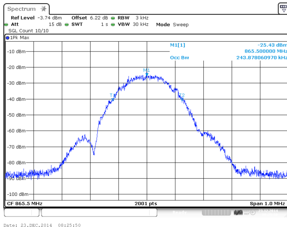
plot 6.3.1.2-#2 Occupied Bandwidth: §90.210, §2.1049; Test results; Downlink; EDGE Input
