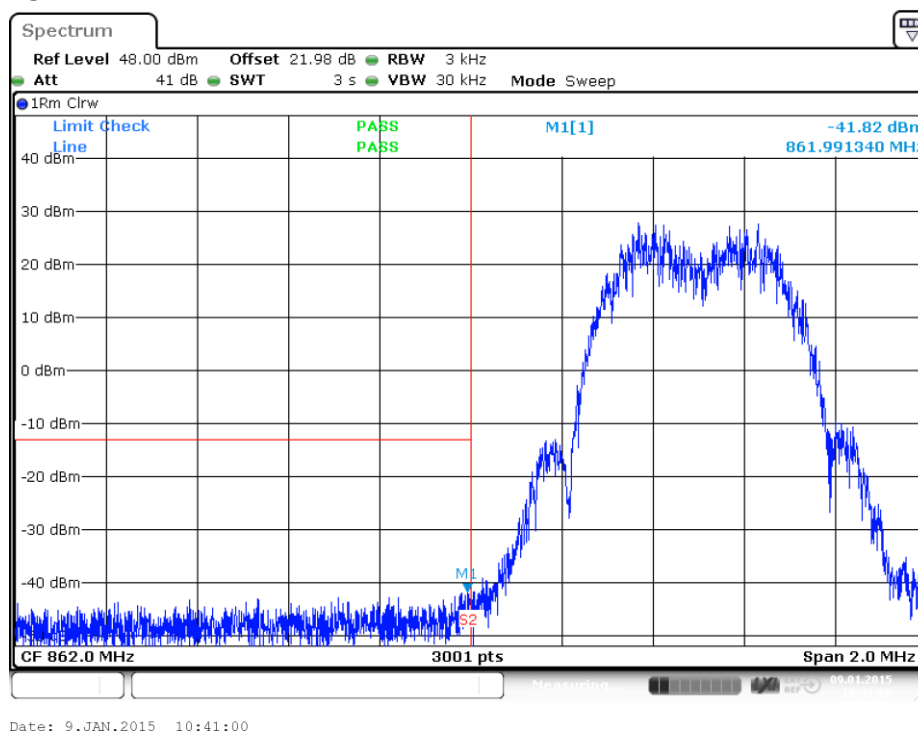
plot 8.3.1.2-#1 Intermodulation: §90.691, §2.1051; Test results; Downlink; EDGE Lower Band Edge
