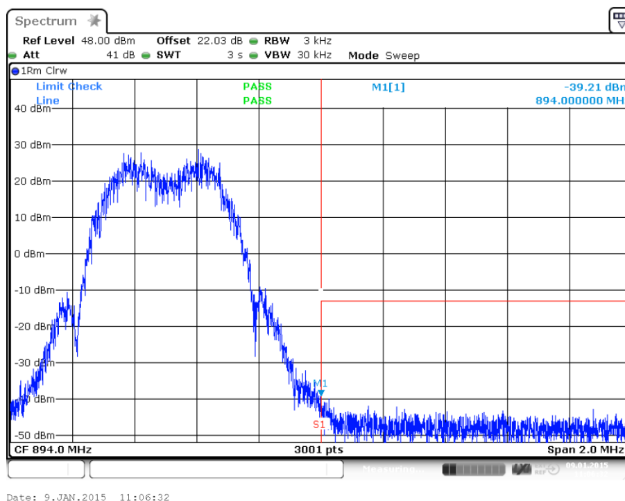
plot 8.3.1.2-#2 Intermodulation: §22.917, §2.1051; Test results; Downlink; EDGE Upper Band Edge
