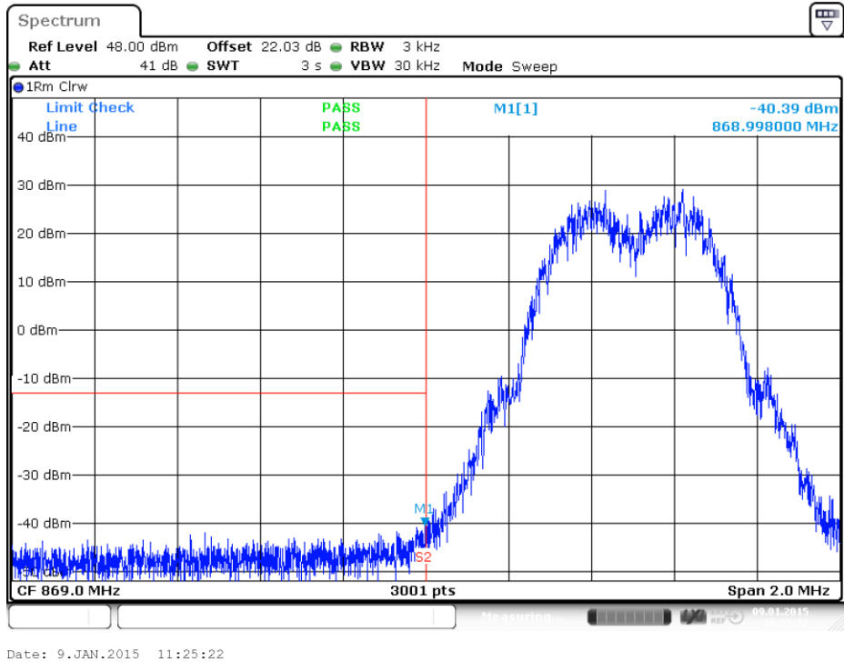
plot 8.3.1.1-#1 Intermodulation: §22.917, §2.1051; Test results; Downlink; GSM Lower Band Edge
