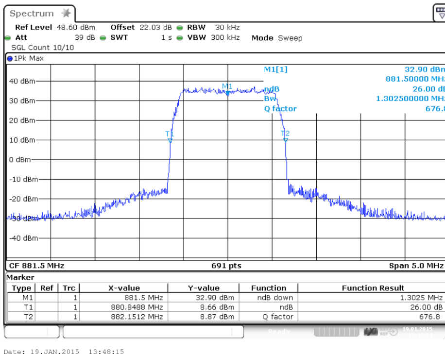
plot 6.3.2.5-#1 Occupied Bandwidth: $2.1049; Test results; 26dB Bandwidth; LTE Output
