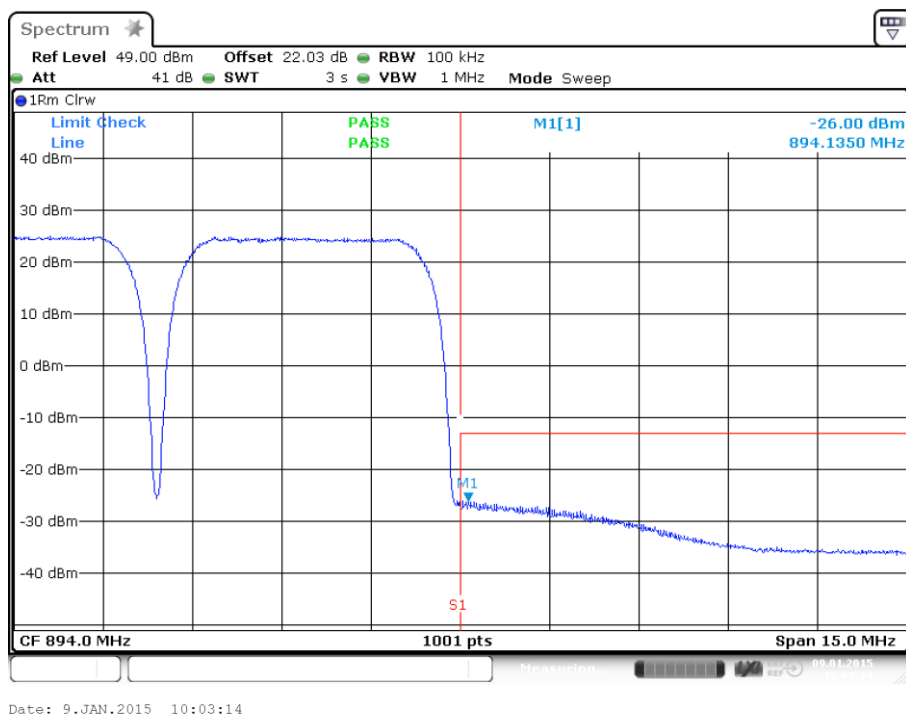
plot 8.3.1.4-#2 Intermodulation: §22.917, §2.1051; Test results; Downlink; WCDMA Upper Band Edge
