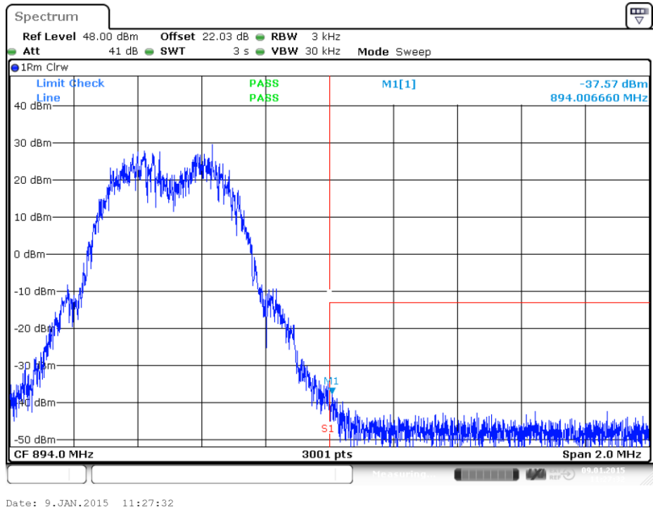
plot 8.3.1.1-#2 Intermodulation: §22.917, §2.1051; Test results; Downlink; GSM Upper Band Edge
