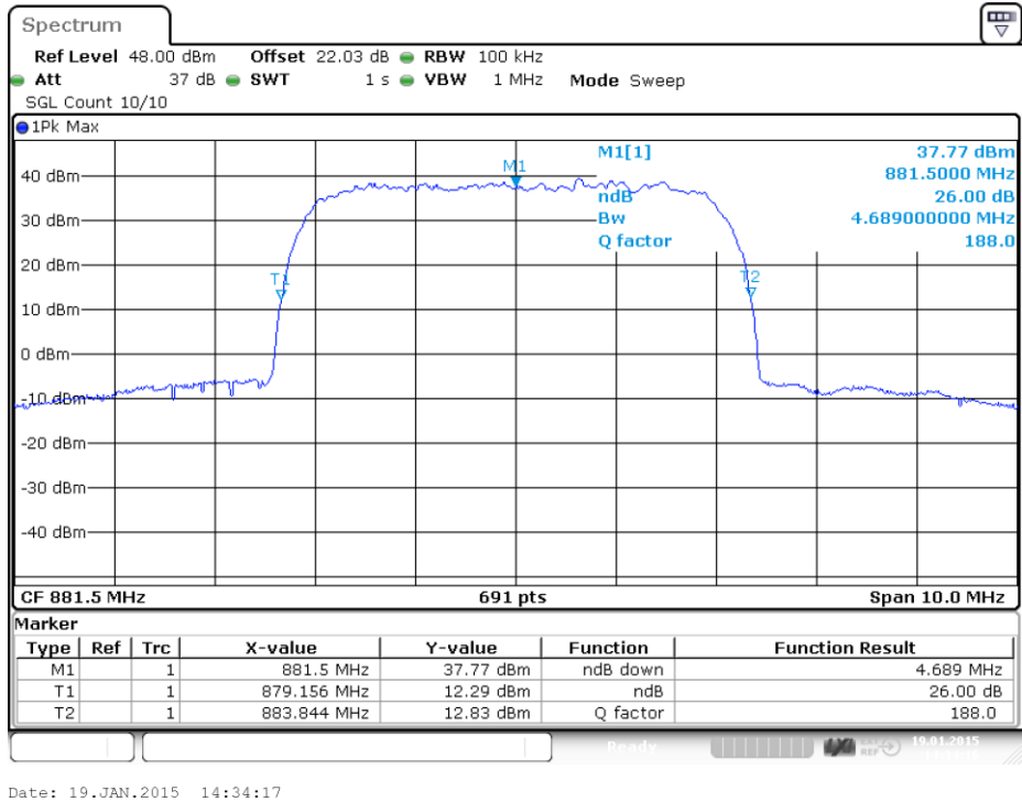
plot 6.3.2.4-#1 Occupied Bandwidth: §2.1049; Test results; 26dB Bandwidth; WCDMA Output
