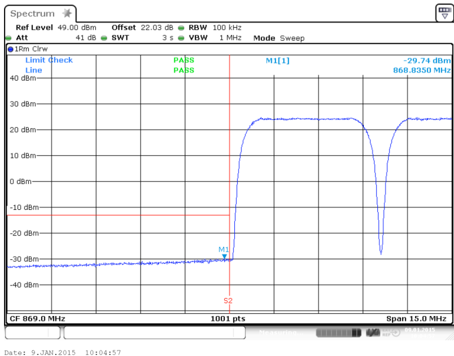
plot 8.3.1.4-#1 Intermodulation: §22.917, §2.1051; Test results; Downlink; WCDMA Lower Band Edge
