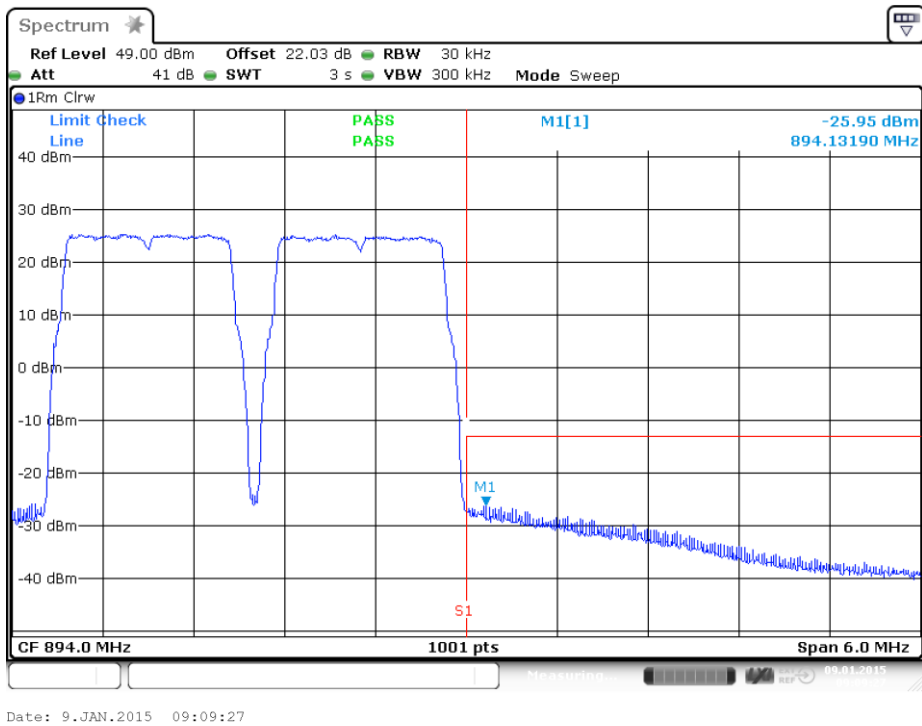
plot 8.3.1.5-#2 Intermodulation: §22.917, §2.1051; Test results; Downlink; LTE Upper Band Edge
