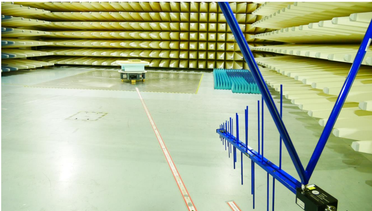
Basic set-up
