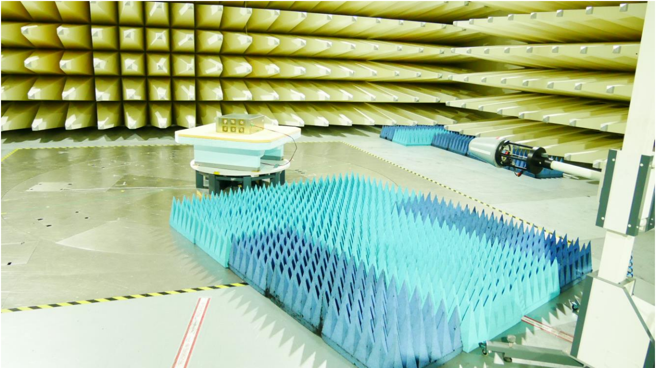
Test setup for radiated emissions in the frequency range 1 – 6 GHz
