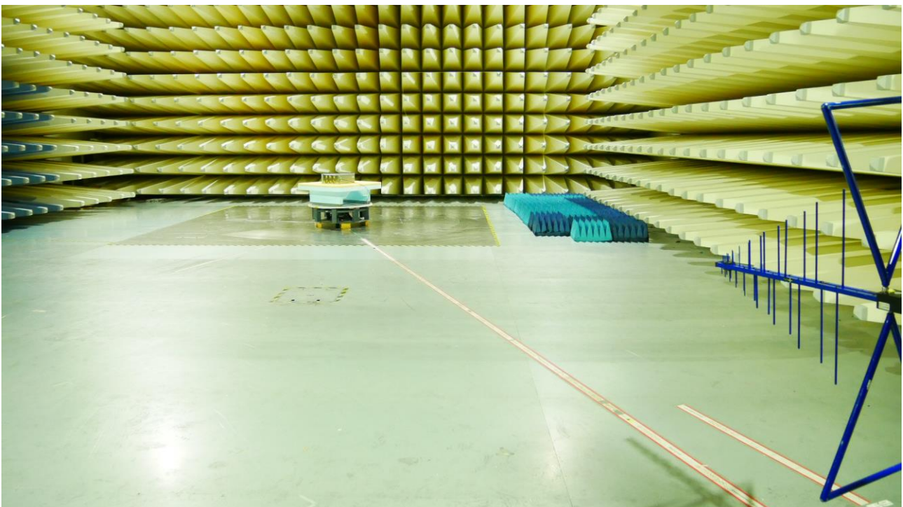
Test setup for radiated emissions in the frequency range 30 – 1000 MHz
