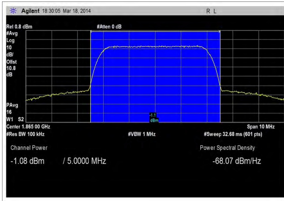
7.2_Max power_UL_1865MHz_AWGN
