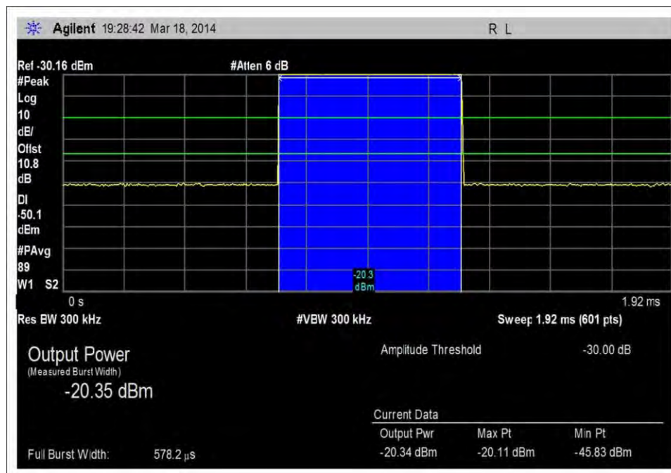
7.2_Max power_DL_877MHz_GSM_RFin=-20dBm
