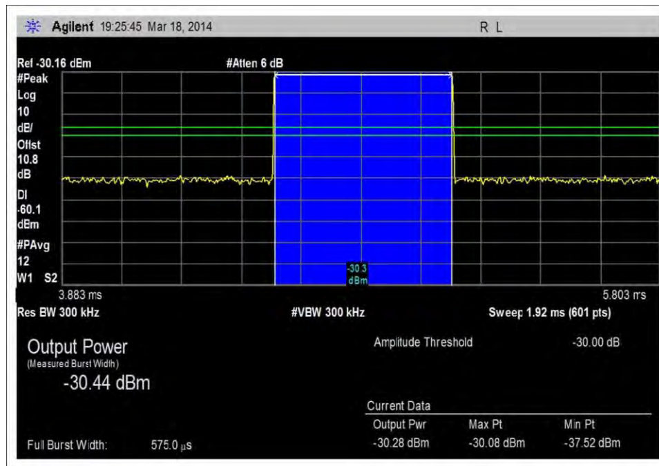
7.2_Max power_DL_877MHz_GSM
