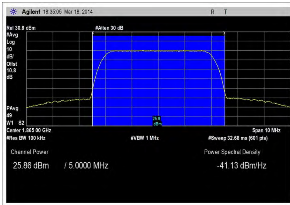
7.2_Max power_UL_1865MHz_AWGN_RFin=27dBm
