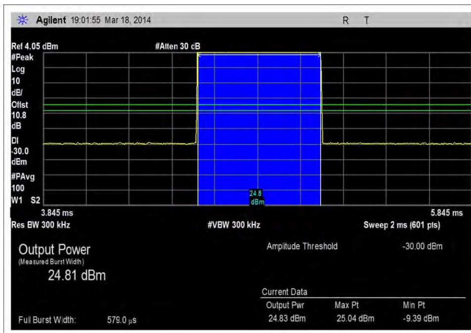
7.2_Max power_UL_1865MHz_GSM_RFin=27dBm
