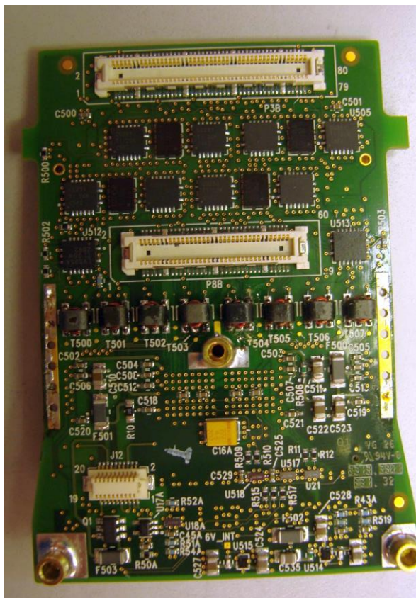
Front End 01314 (shields removed)
