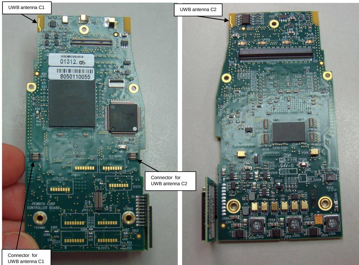
TOP view
