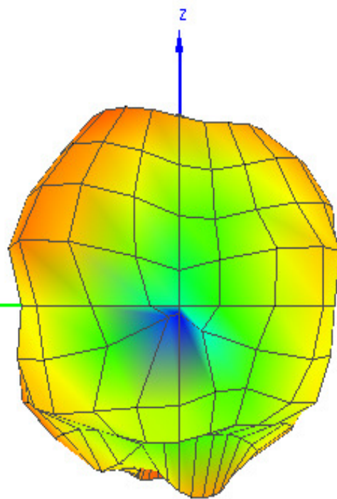
Theta = 90, Phi = 180
