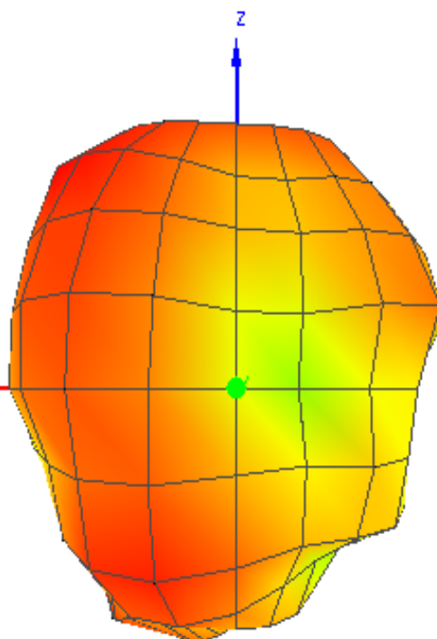
Theta = 90, Phi = 90
