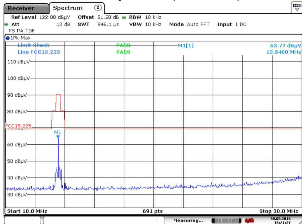
NFC Field strength of emission (10 MHz to 30 MHz)
