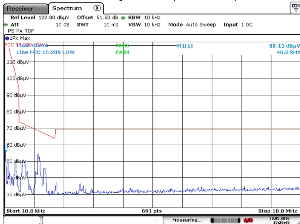
NFC Field strength of emission (10 kHz to 10 MHz)
