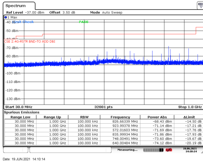
Figure 8.2-17: Conducted spurious emission within restricted band 30 MHz to 1 GHz, BLE TX on high channel
