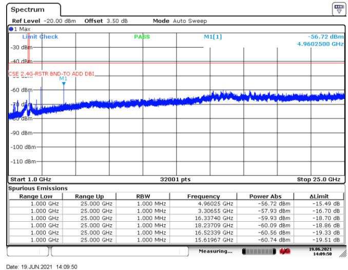
Figure 8.2-18: Conducted spurious emission within restricted band above 1 GHz, BLE TX on high channel
