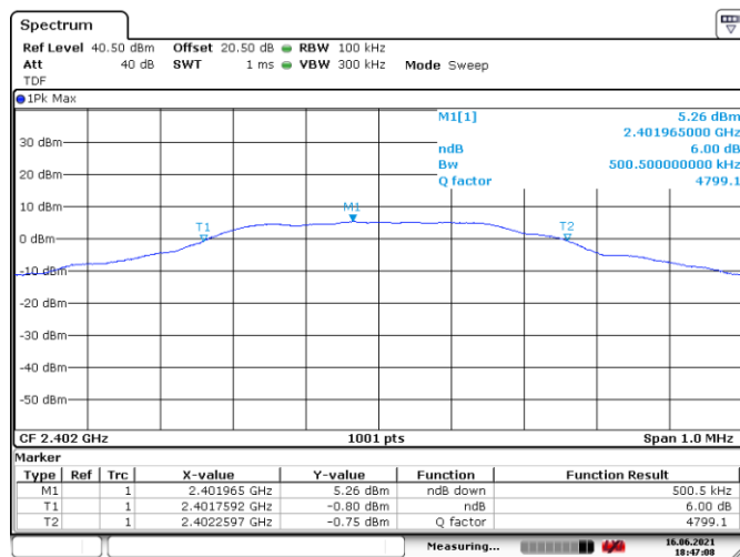
Figure 8.5-1: 6 dB bandwidth on BLE, Tx low channel
