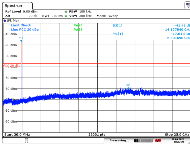
Figure 8.7-3: Conducted spurious emissions outside restricted band, TX on Low channel
