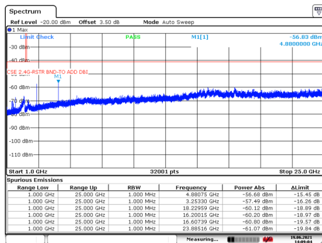
Figure 8.7-13: Conducted spurious emission within restricted band above 1 GHz, TX on mid channel
