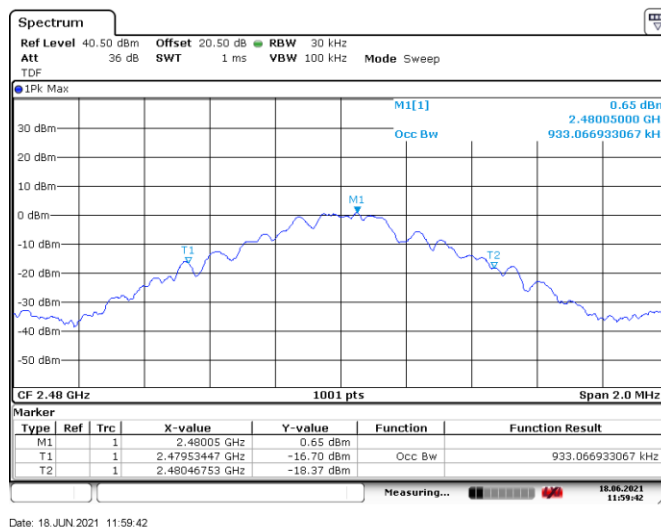
Figure 8.5-6: 99% bandwidth on BLE, Tx high channel
