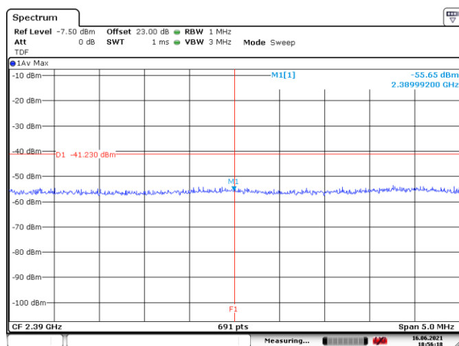
Figure 8.7-8: Conducted spurious emission at band edge within restricted band, TX on low channel, average
