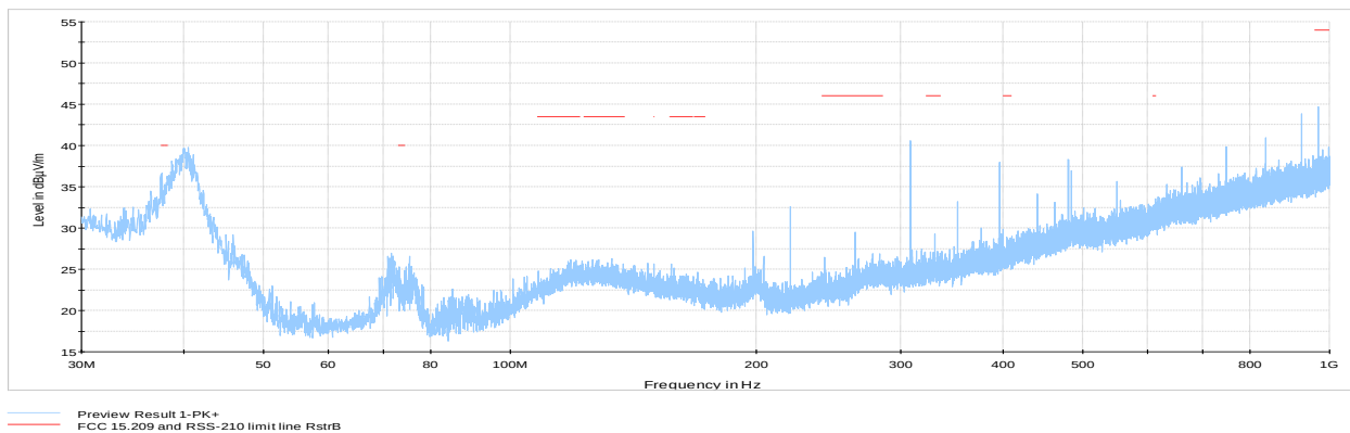
Figure 8.7-18: Cabinet Radiated spurious emissions 30 MHz to 1 GHz, High channel
