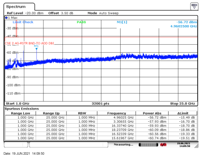
Figure 8.7-15: Conducted spurious emission within restricted band above 1 GHz, TX on high channel
