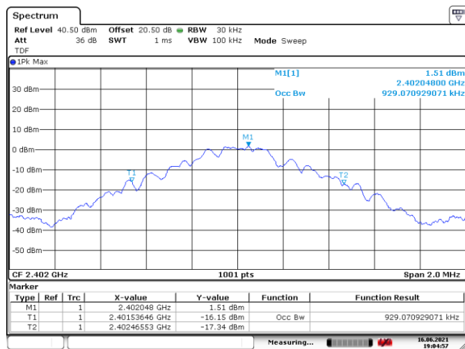
Figure 8.5-4: 99% bandwidth on BLE, Tx low channel
