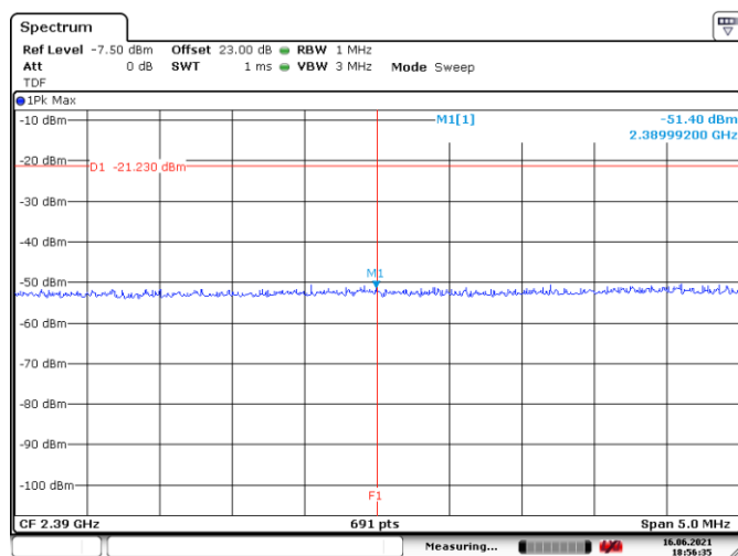
Figure 8.7-6: Conducted spurious emission at band edge within restricted band, TX on low channel, Peak
