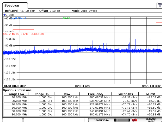
Figure 8.7-10: Conducted spurious emission within restricted band 30 MHz to 1 GHz, TX on low channel
