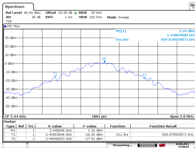
Figure 8.5-5: 99% bandwidth on BLE, Tx mid channel
