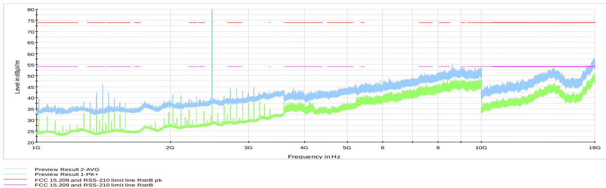
Figure 8.7-21: Cabinet Radiated spurious emissions 1 to 18 GHz, High channel
