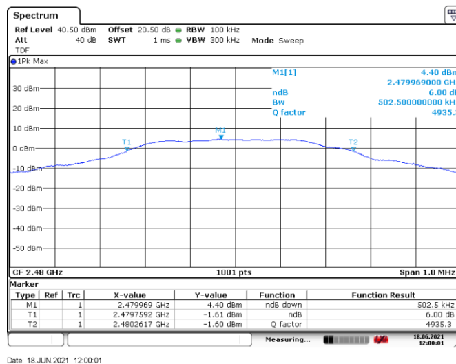
Figure 8.5-3: 6 dB bandwidth on BLE, Tx high channel
