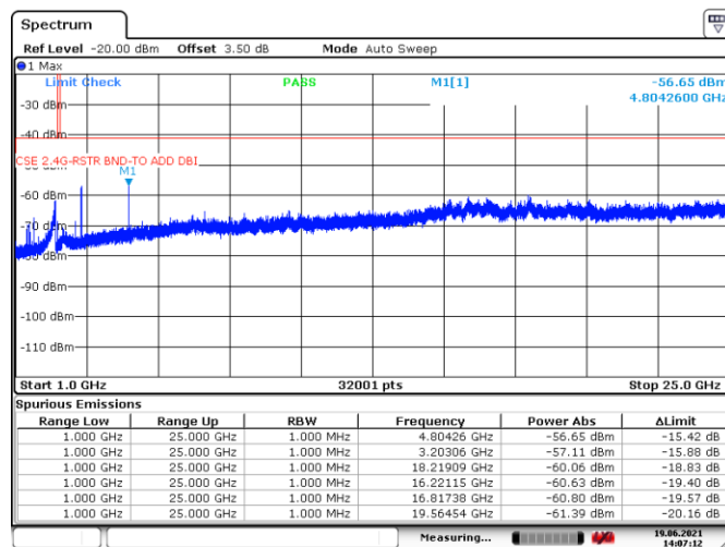
Figure 8.7-11: Conducted spurious emission within restricted band above 1 GHz, TX on low channel
