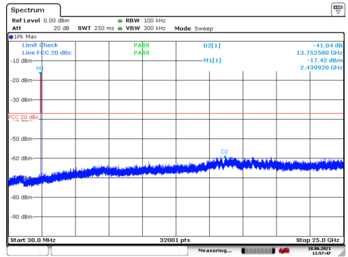
Figure 8.7-4: Conducted spurious emissions outside restricted band, TX on Mid channel
