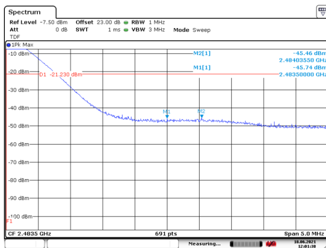
Figure 8.7-7: Conducted spurious emissions at band edge within restricted band, TX on High channel, Peak
