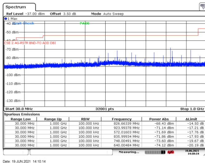
Figure 8.7-14: Conducted spurious emission within restricted band 30 MHz to 1 GHz, TX on high channel
