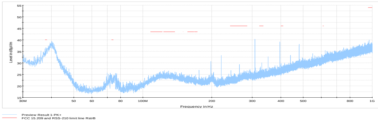
Figure 8.7-16: Cabinet Radiated spurious emissions 30 MHz to 1 GHz, Low channel
