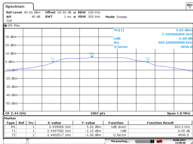
Figure 8.5-2: 6 dB bandwidth on BLE, Tx mid channel
