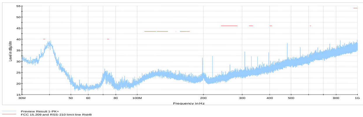
Figure 8.7-17: Cabinet Radiated spurious emissions 30 MHz to 1 GHz, mid channel
