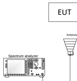
Figure 5.6-1: Radiated testing block diagram
