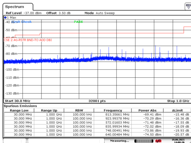
Figure 8.7-12: Conducted spurious emission within restricted band 30 MHz to 1 GHz, TX on mid channel
