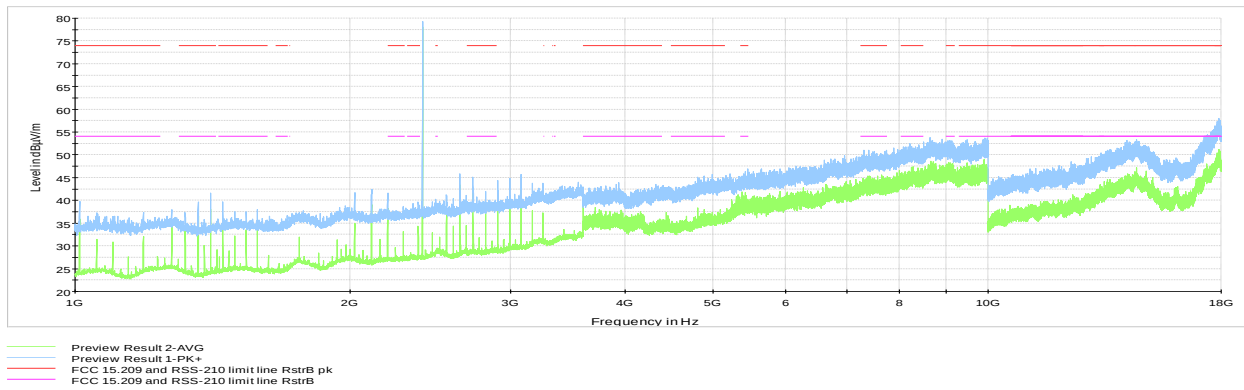
Figure 8.7-19: Cabinet Radiated spurious emissions 1 to 18 GHz, Low channel
