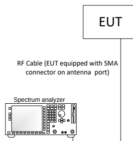
Figure 5.6-2: Antenna port testing block diagram
