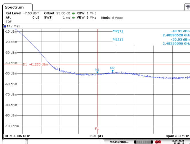
Figure 8.7-9: Conducted spurious emissions at band edge within restricted band, TX on High channel, average
