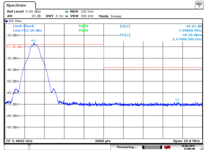
Figure 8.7-2: Conducted spurious emissions at band edge outside restricted band, TX on High channel
