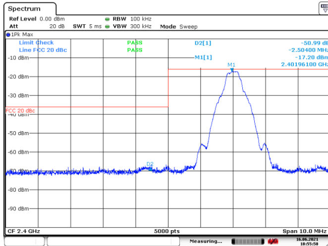
Figure 8.7-1: Conducted spurious emission at band edge outside restricted band, TX on low channel
