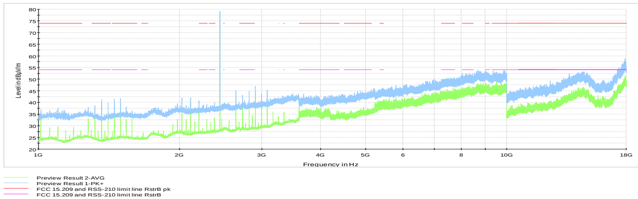
Figure 8.7-20: Cabinet Radiated spurious emissions 1 to 18 GHz, mid channel
