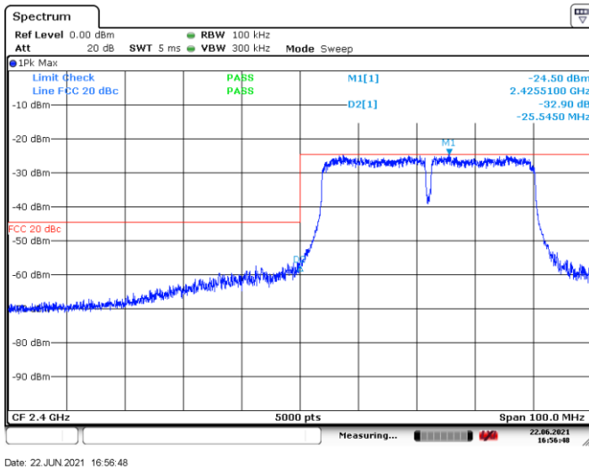
Figure 8.7-7: Conducted spurious emission at band edge outside restricted band, TX on 802.11n HT40 low channel
