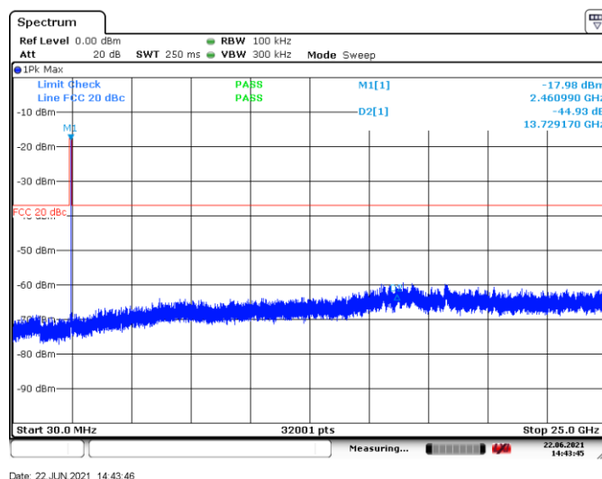
Figure 8.7-11: Conducted spurious emissions outside restricted band, TX on 802.11b High channel
