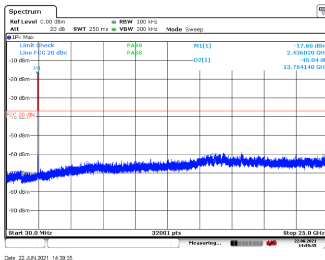
Figure 8.7-10: Conducted spurious emissions outside restricted band, TX on 802.11b Mid channel
