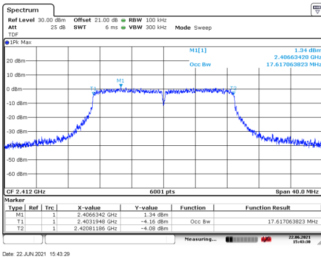
Figure 8.5-7: 99% bandwidth on 802.11n HT20, sample plot
