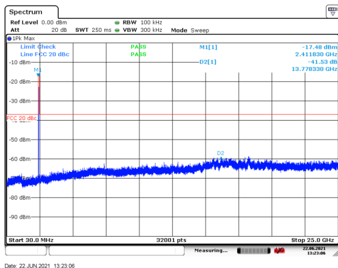
Figure 8.7-9: Conducted spurious emissions outside restricted band, TX on 802.11b Low channel
