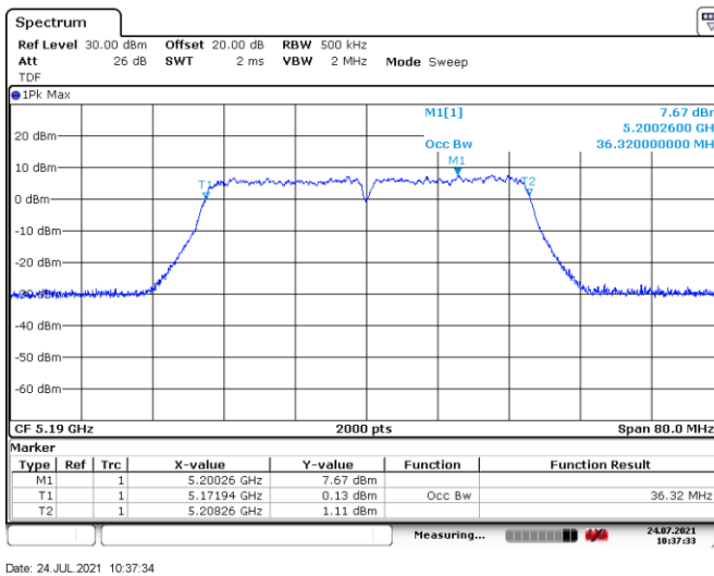
Figure 8.6-3: 99% bandwidth on 802.11n HT40/802.11ac VHT40, sample plot
