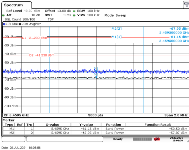
Figure 8.8-14: Lower band edge, Tx on low channel, 802.11n HT20/802.11ac VHT20
