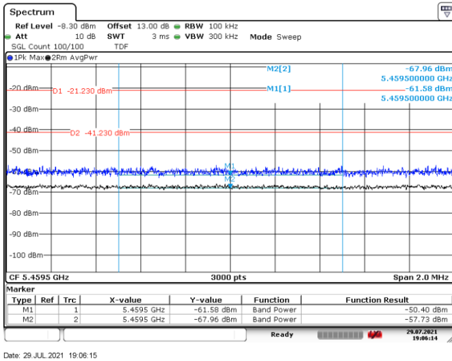
Figure 8.8-12: Lower band edge, Tx on low channel, 802.11a
