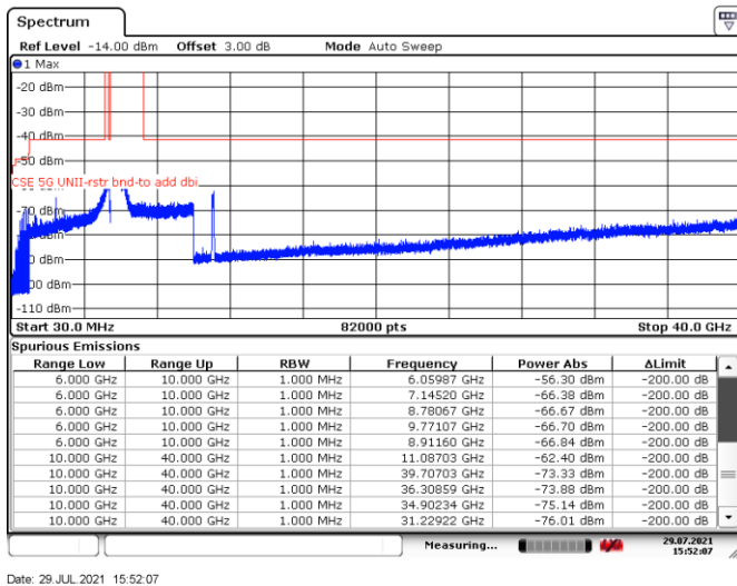
Figure 8.8-29: Spurious emissions within restricted bands, Tx on low channel, 802.11ac VHT80
