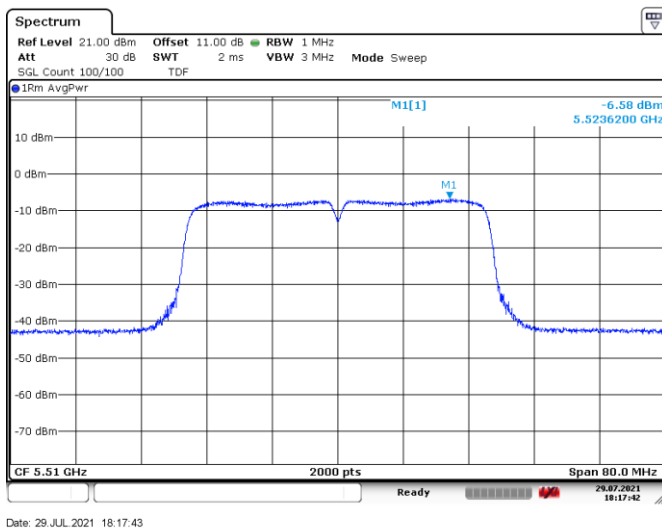
Figure 8.7-3: Sample plot for PSD on 802.11n HT40/802.11ac VHT40
