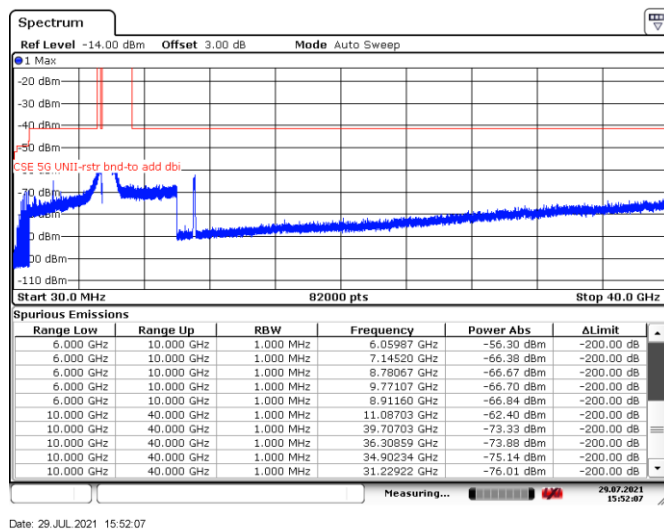
Figure 8.2-94: Spurious emissions within restricted bands, Tx on UNII-2c low channel, 802.11ac VHT80
