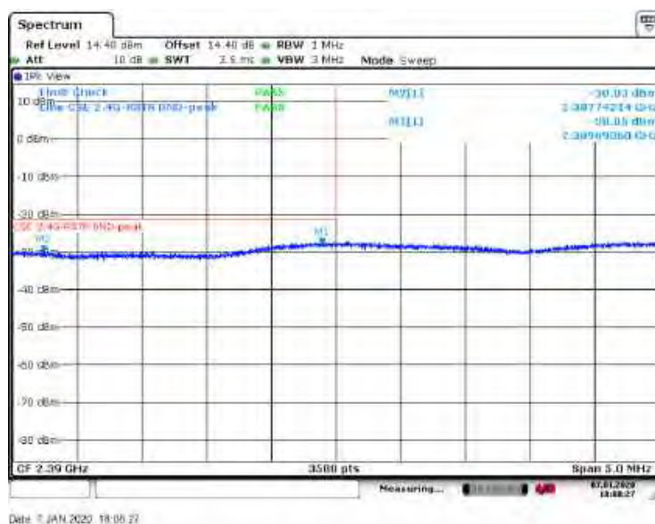
Figure 8.7-25: Restricted Band Edge emissions for low channel, Peak
