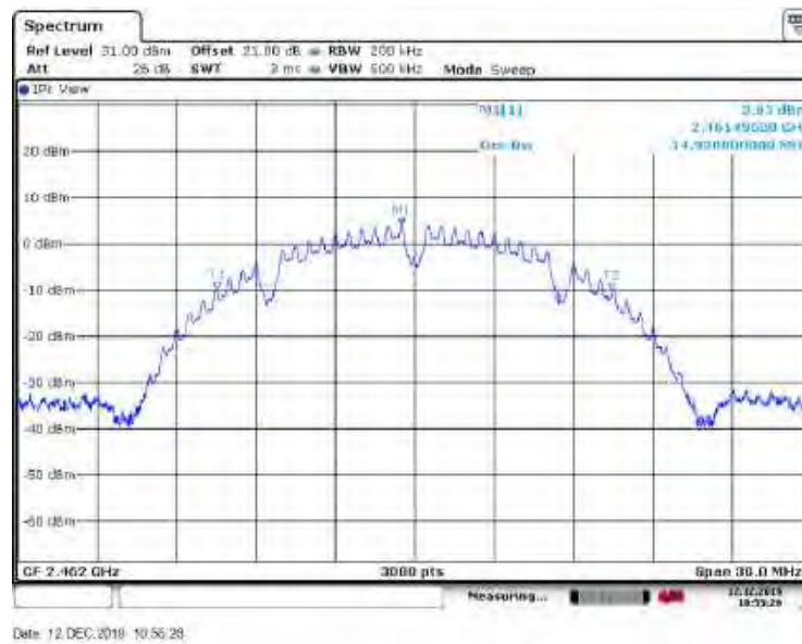
Figure 8.5-6: 99% occupied bandwidth on high channel, sample plot
