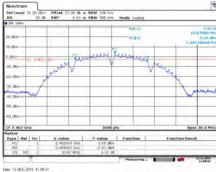
Figure 8.5-3: 6 dB bandwidth on high channel, sample plot
