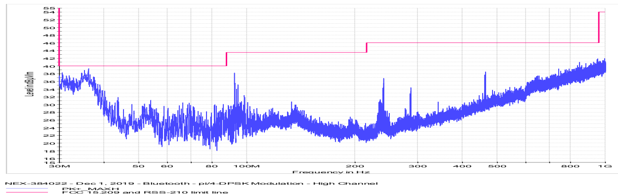
Figure 8.7-34: Radiated spurious emissions for high channel 30 MHz to 1 GHz
