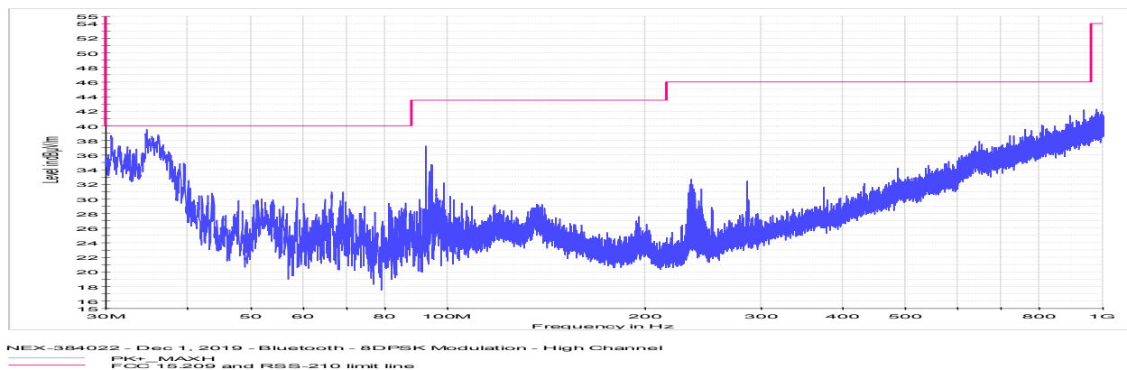
Figure 8.7-37: Radiated spurious emissions for high channel 30 MHz to 1 GHz
