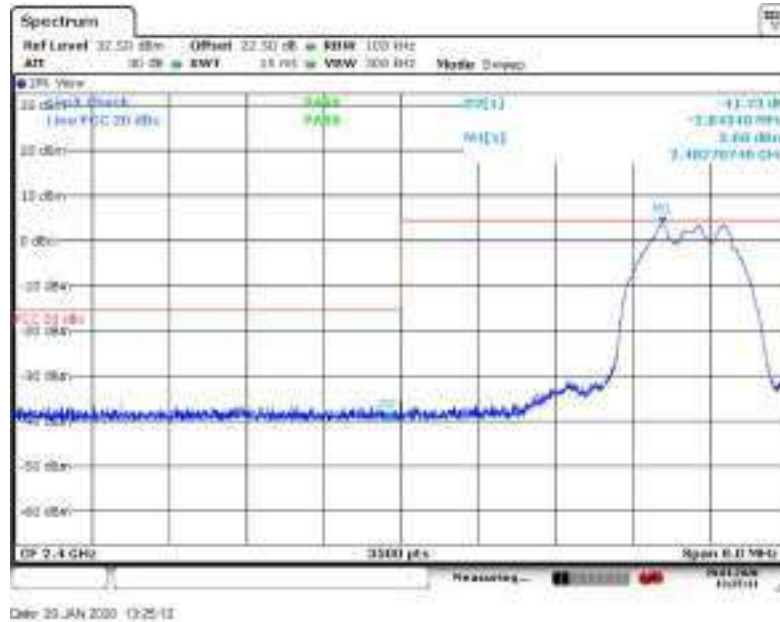
Figure 8.7-17: Band Edge emissions for low channel
