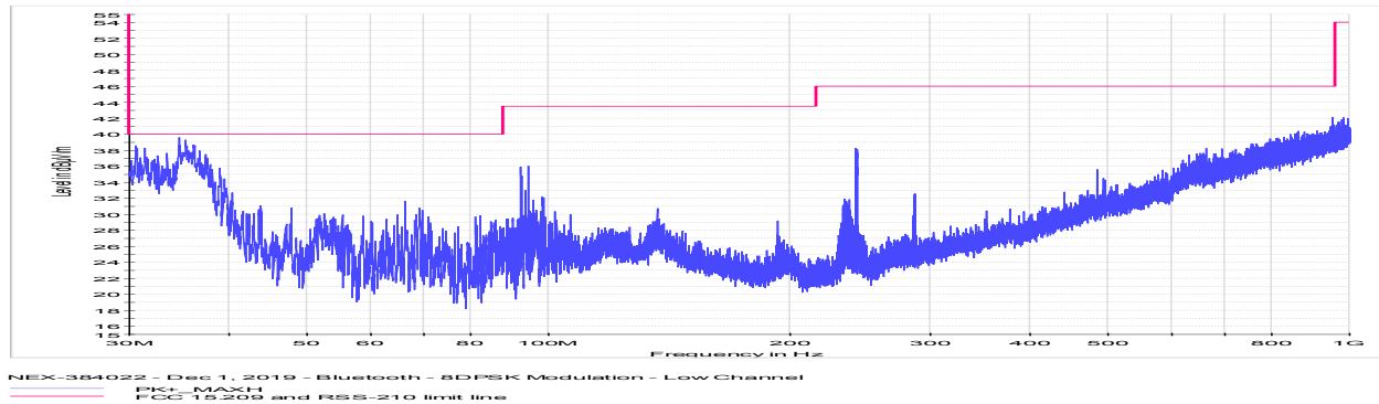
Figure 8.7-35: Radiated spurious emissions for low channel 30 MHz to 1 GHz
