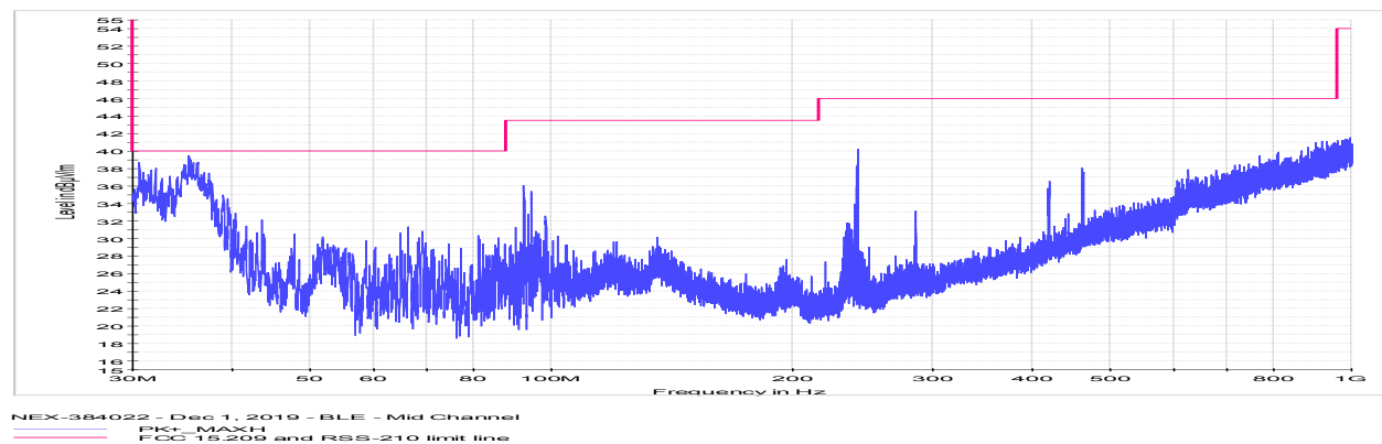
Figure 8.7-39: Radiated spurious emissions for mid channel 30 MHz to 1 GHz
