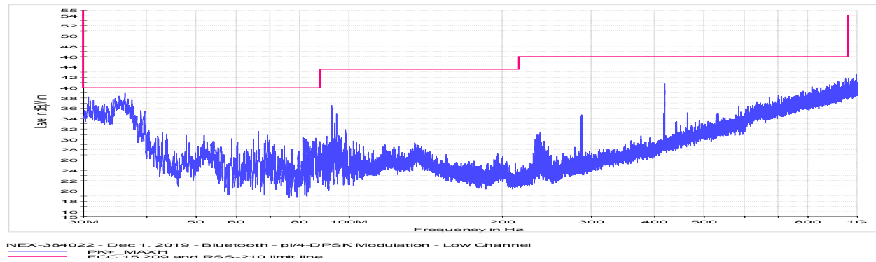
Figure 8.7-32: Radiated spurious emissions for low channel 30 MHz to 1 GHz
