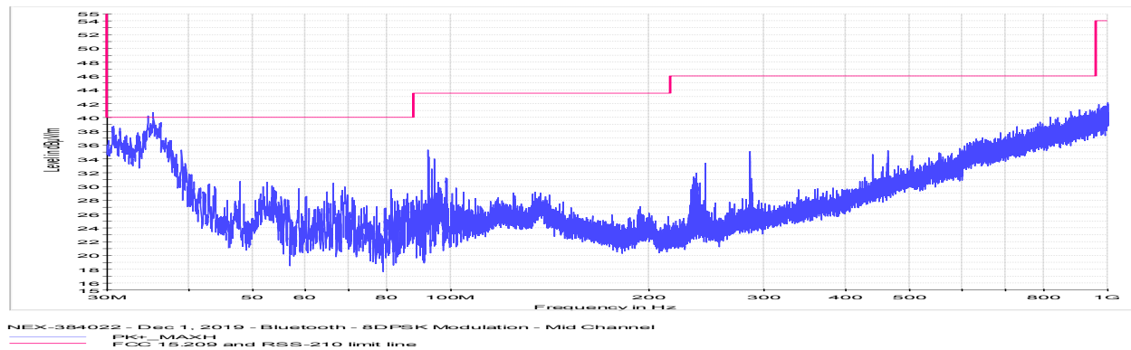
Figure 8.7-36: Radiated spurious emissions for mid channel 30 MHz to 1 GHz
