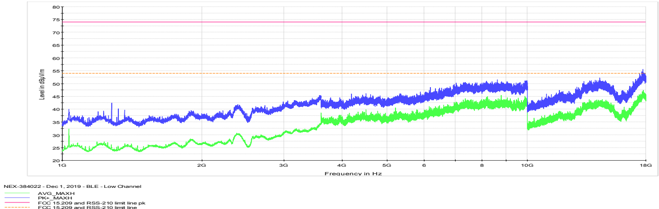
Figure 8.7-44: Radiated spurious emissions for low channel 1 GHz to 18 GHz
