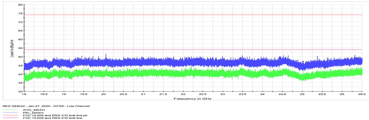
Figure 8.7-45: Radiated spurious emissions for low channel 18 GHz to 26.5 GHz
