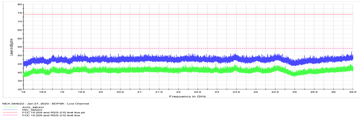
Figure 8.7-47: Radiated spurious emissions for low channel 18 GHz to 26.5 GHz
