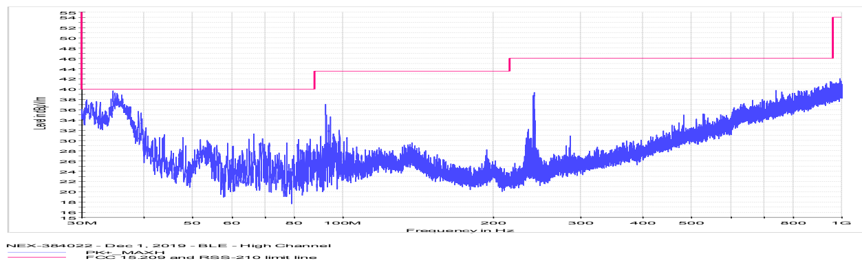
Figure 8.7-40: Radiated spurious emissions for high channel 30 MHz to 1 GHz
