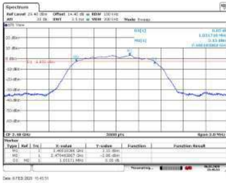
Figure 8.5-9: 6 dB bandwidth on high channel
