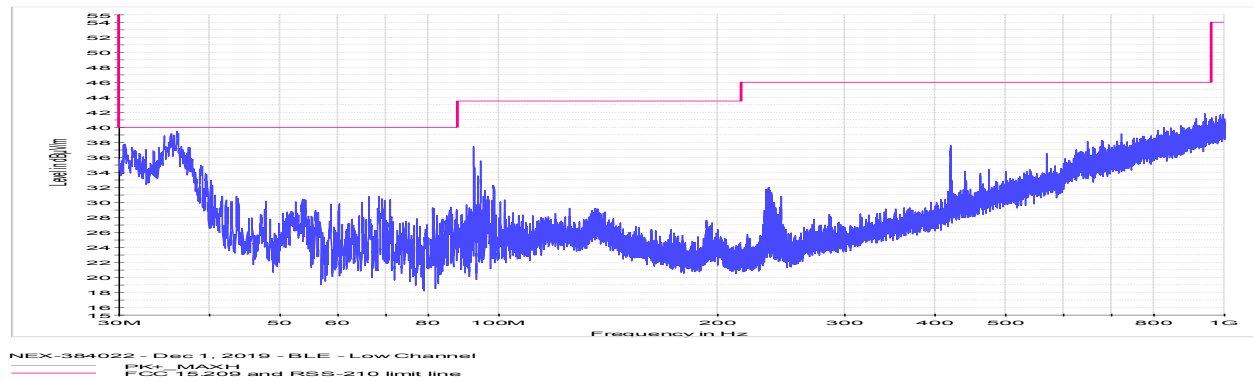
Figure 8.7-38: Radiated spurious emissions for low channel 30 MHz to 1 GHz
