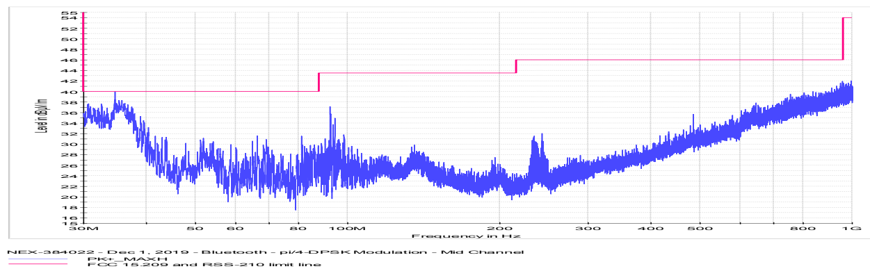
Figure 8.7-33: Radiated spurious emissions for mid channel 30 MHz to 1 GHz
