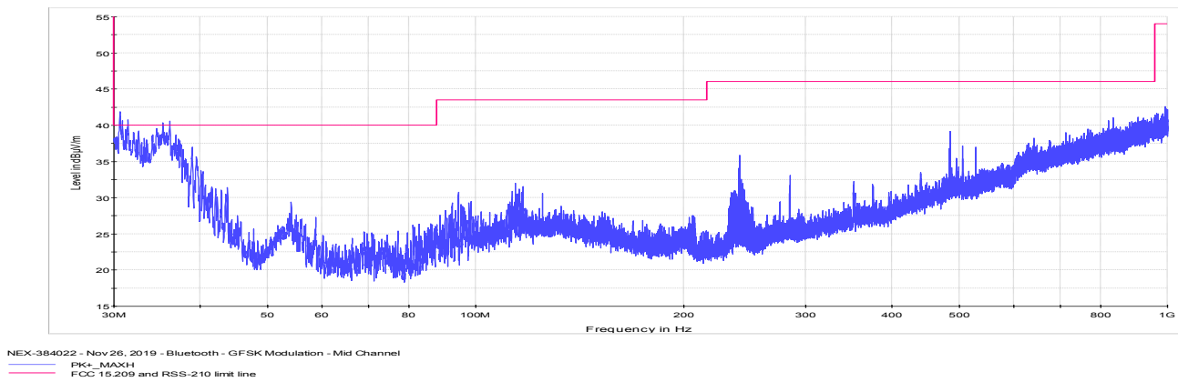
Figure 8.7-30: Radiated spurious emissions for mid channel 30 MHz to 1 GHz
