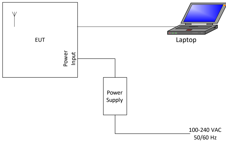
Figure 3.6-1: Setup diagram
