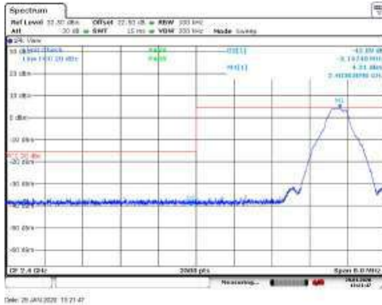
Figure 8.7-13: Band Edge emissions for low channel
