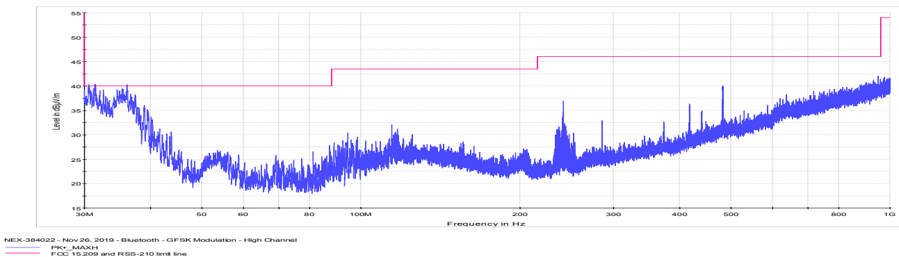
Figure 8.7-31: Radiated spurious emissions for high channel 30 MHz to 1 GHz
