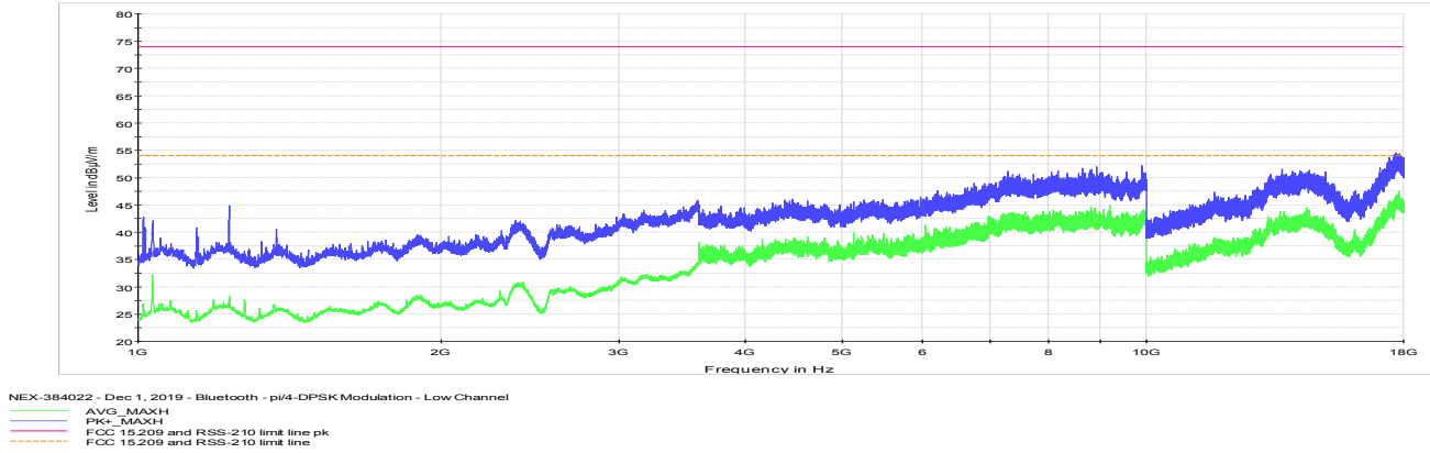
Figure 8.7-42: Radiated spurious emissions for low channel 1 GHz to 18 GHz
