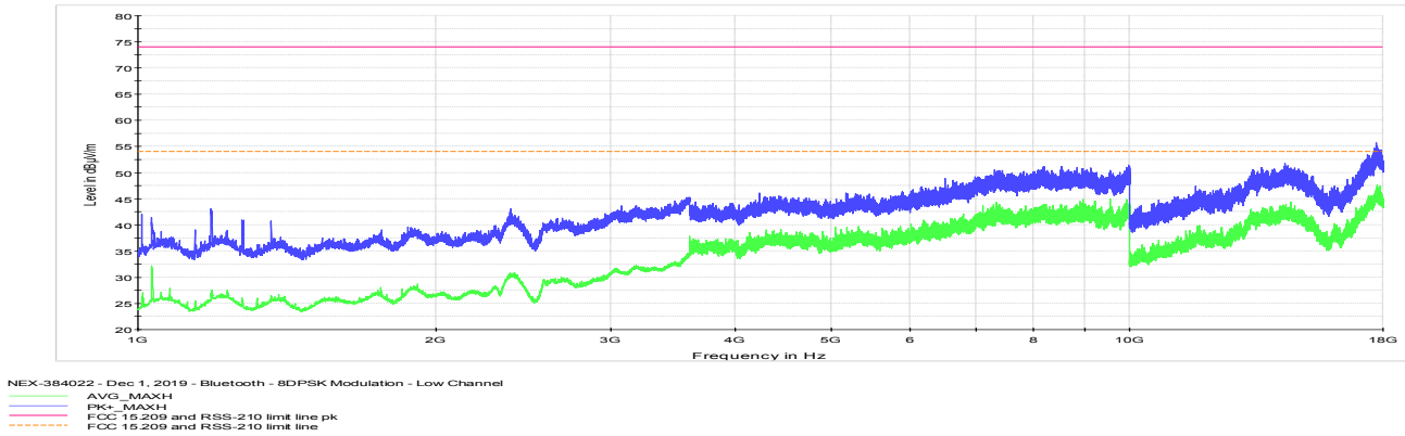
Figure 8.7-43: Radiated spurious emissions for low channel 1 GHz to 18 GHz
