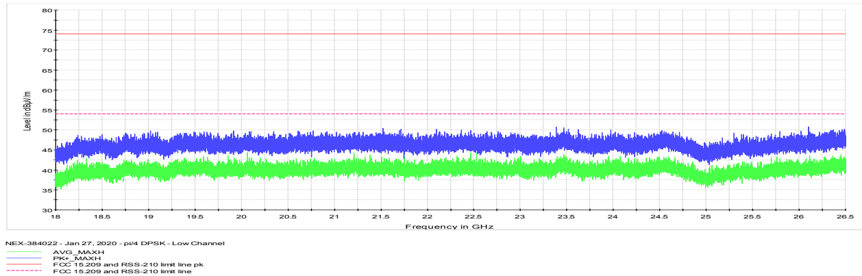
Figure 8.7-46: Radiated spurious emissions for low channel 18 GHz to 26.5 GHz
