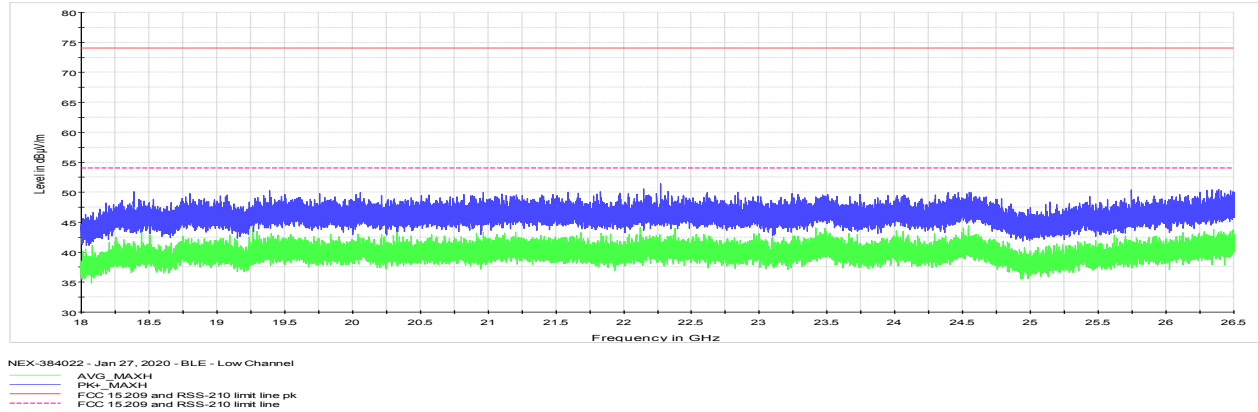
Figure 8.7-48: Radiated spurious emissions for low channel 18 GHz to 26.5 GHz
