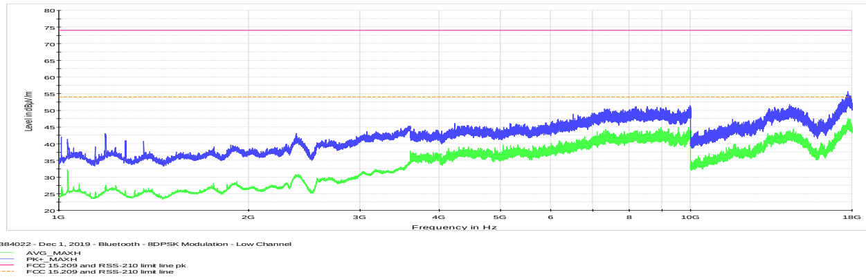
Figure 8.7-55: Radiated spurious emissions for low channel 1 GHz to 18 GHz
