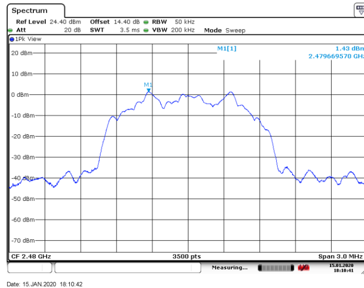
Figure 8.8-9: PSD sample plot on high channel
