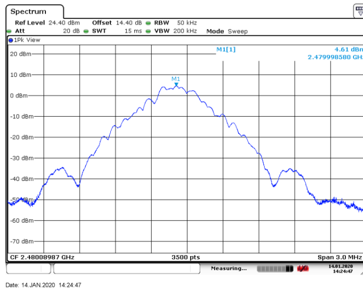
Figure 8.8-3: PSD sample plot on high channel
