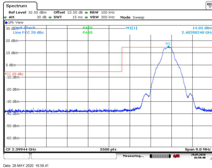
Figure 8.7-31: Band Edge emissions for low channel
