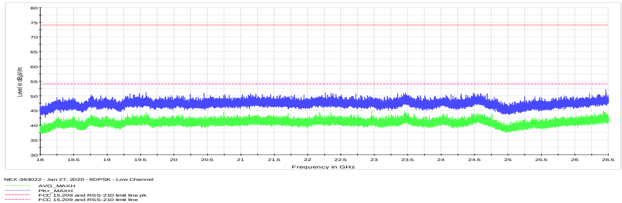
Figure 8.7-59: Radiated spurious emissions for low channel 18 GHz to 26.5 GHz
