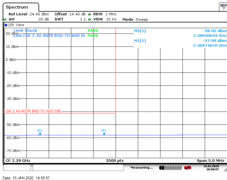
Figure 8.7-40: Restricted Band Edge emissions for low channel, Average
