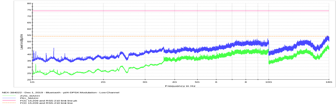
Figure 8.7-54: Radiated spurious emissions for low channel 1 GHz to 18 GHz
