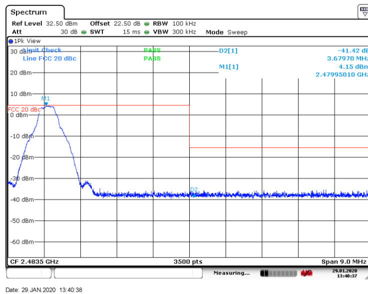
Figure 8.7-32: Band Edge emissions for high channel
