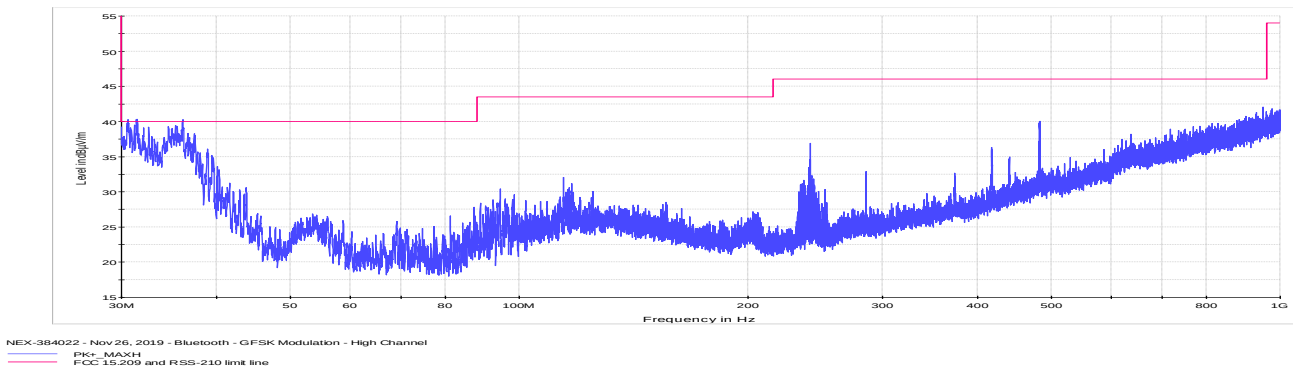
Figure 8.7-43: Radiated spurious emissions for high channel 30 MHz to 1 GHz
