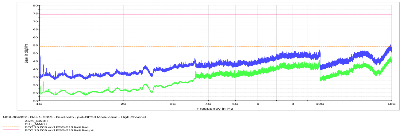
Figure 8.1 1: Radiated spurious emissions for high channel 1 GHz to 18 GHz
