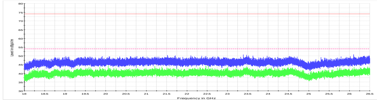
Figure 8.7-58: Radiated spurious emissions for low channel 18 GHz to 26.5 GHz
