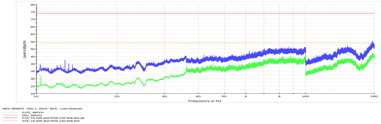
Figure 8.7-56: Radiated spurious emissions for low channel 1 GHz to 18 GHz
