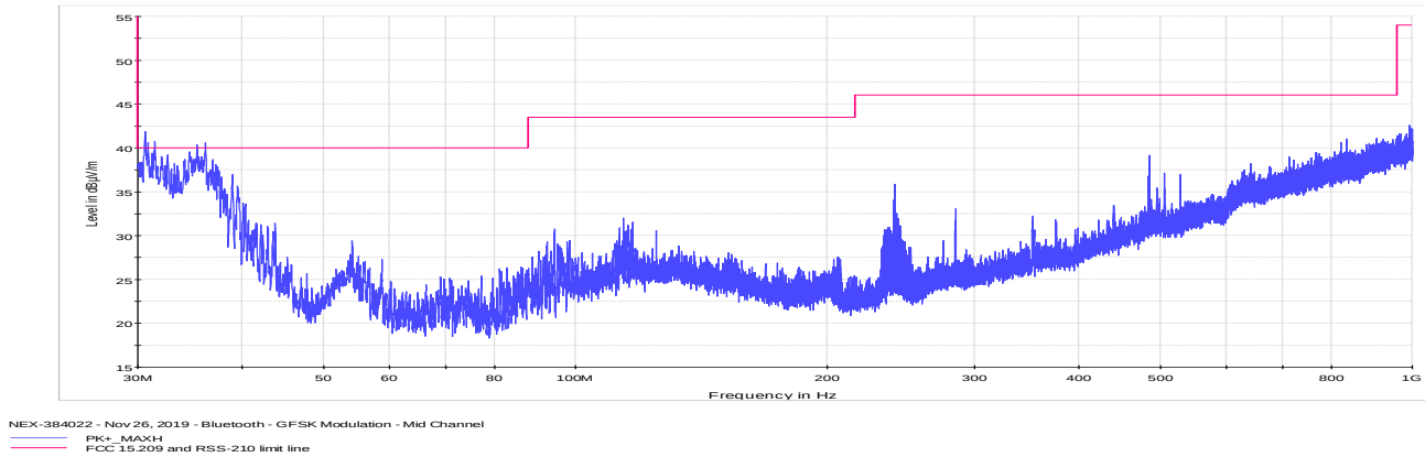
Figure 8.7-42: Radiated spurious emissions for mid channel 30 MHz to 1 GHz
