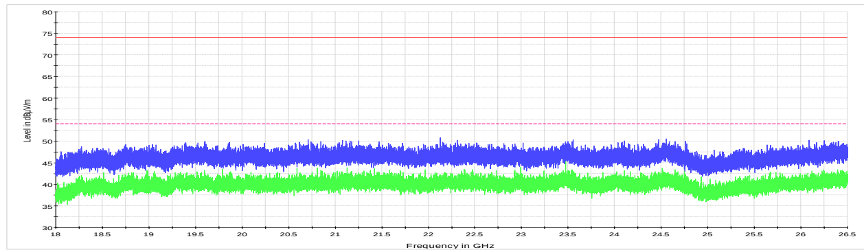
Figure 8.7-58: Radiated spurious emissions for low channel 18 GHz to 26.5 GHz
