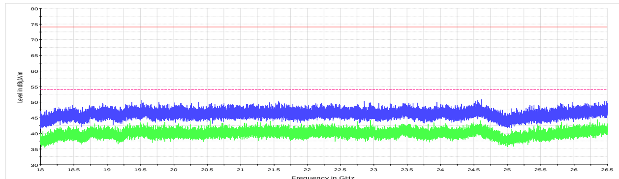
Figure 8.1 1: Radiated spurious emissions for mid channel 18 GHz to 26.5 GHz
