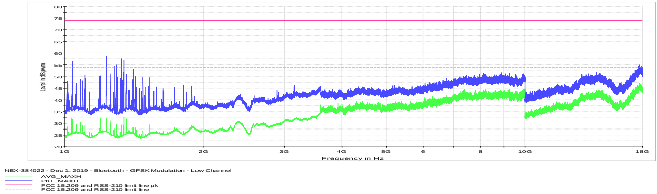
Figure 8.7-53: Radiated spurious emissions for low channel 1 GHz to 18 GHz
