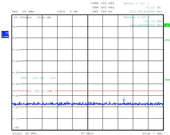
Figure 8.4-13: Conducted spurious emissions outside restricted bands for 802.11b, below 1 GHz, mid channel
