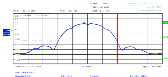
Figure 8.3-1: Output power on 802.11b, sample plot
