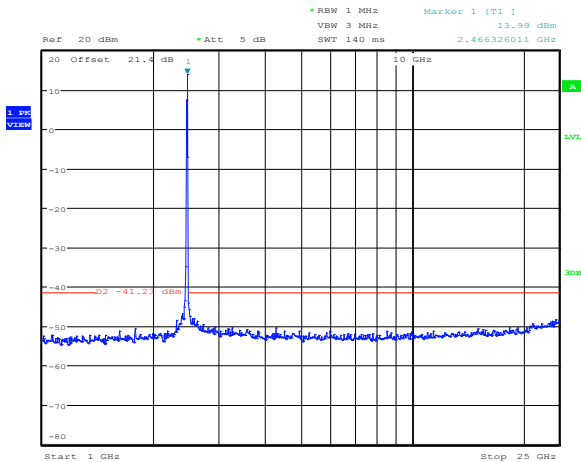
Figure 8.4-14: Conducted spurious emissions outside restricted bands for 802.11b, above 1 GHz, mid channel
