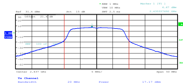
Figure 8.3-2: Output power on 802.11g, sample plot
