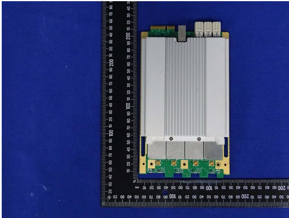
(1) EUT Photo (M/N: SDR-2400)
