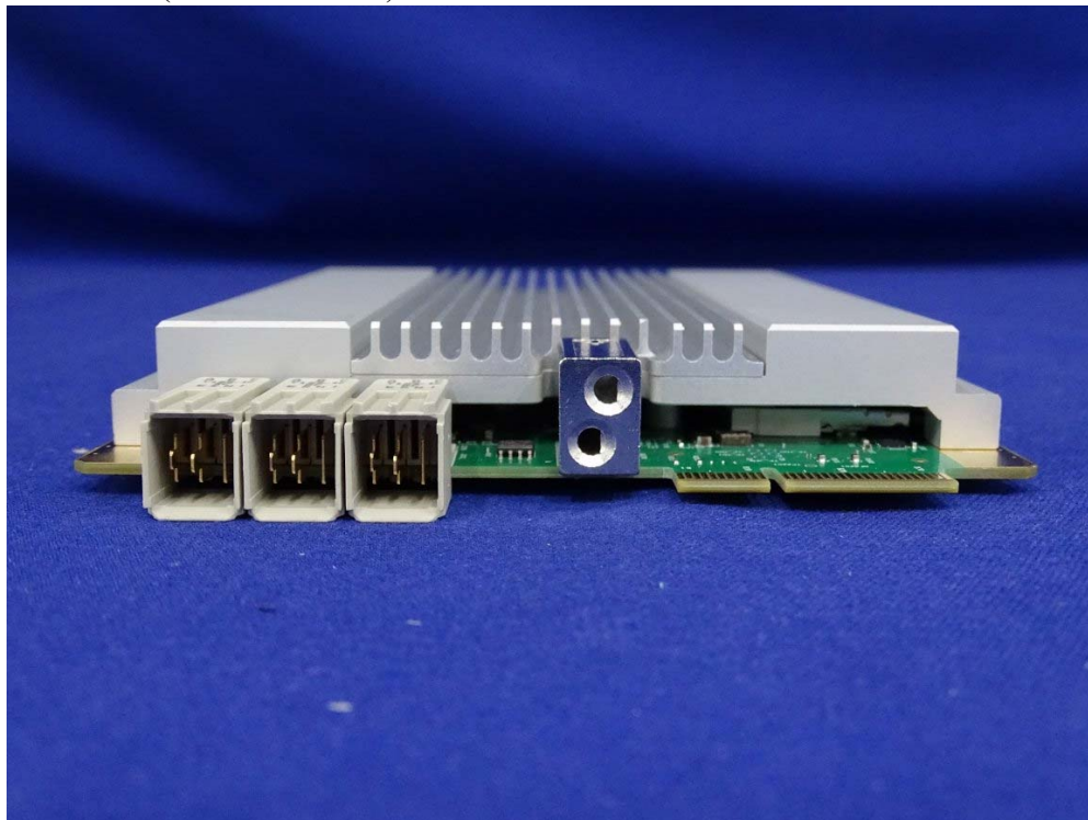
(9) EUT Photo (M/N: SDR-2400)
