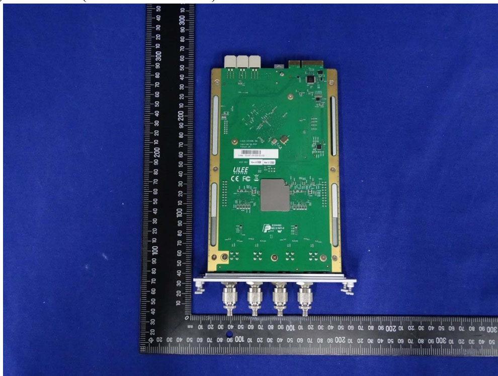
(12) EUT Photo (M/N: SM-SDR-2400)
