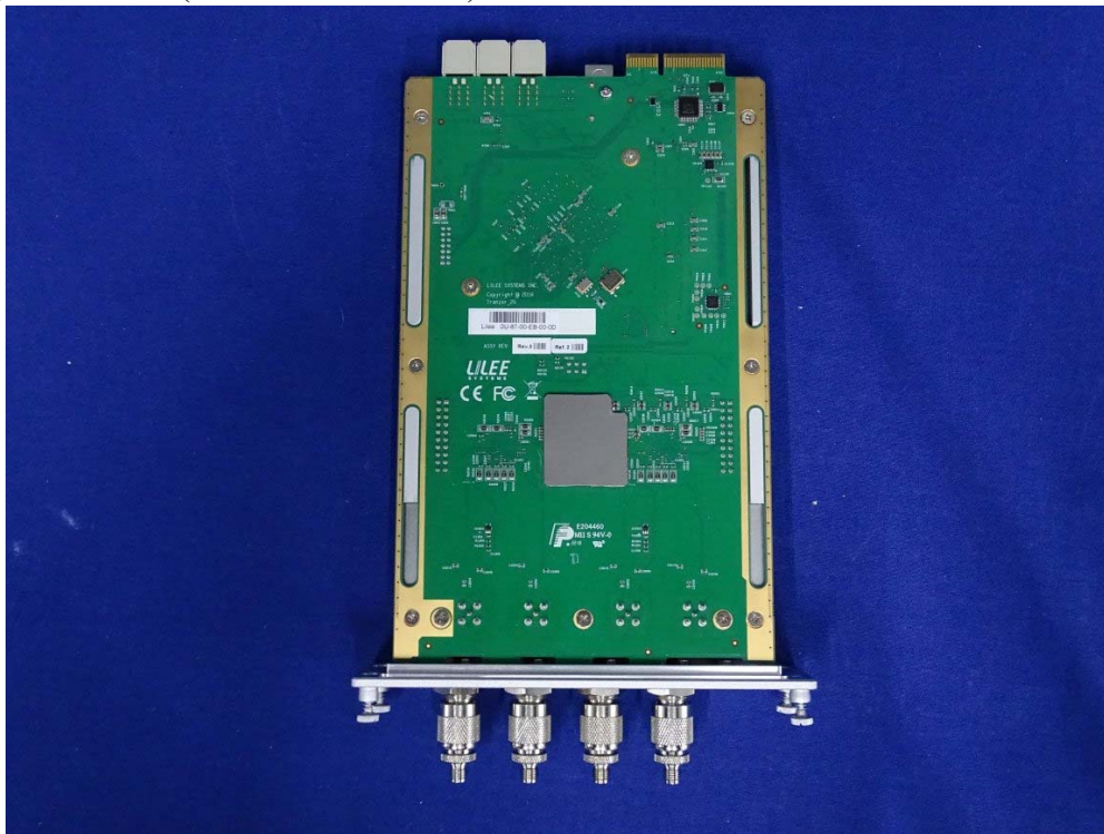
(22) EUT Photo (M/N: SM-SDR-2400)
