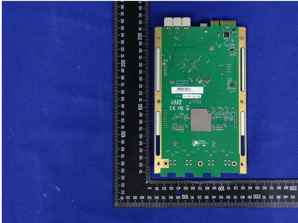
(2) EUT Photo (M/N: SDR-2400)
