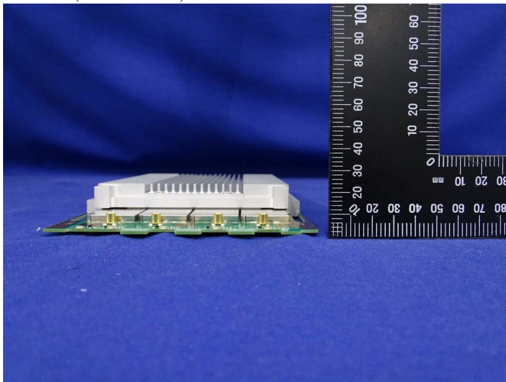
(6) EUT Photo (M/N: SDR-2400)
