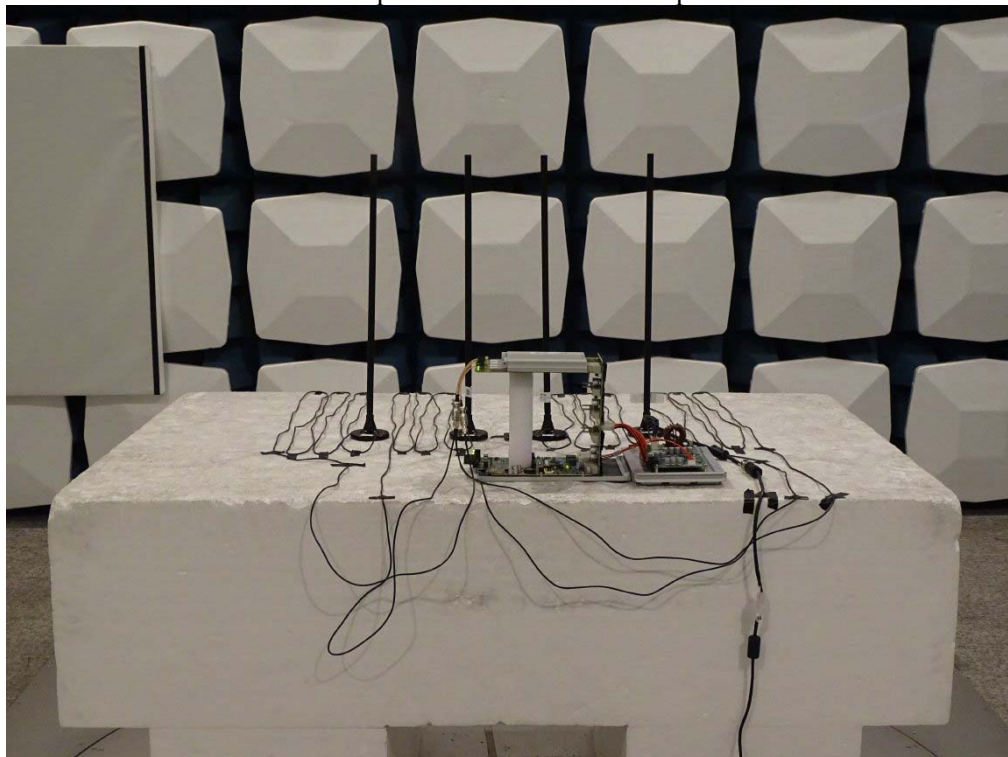
Back View of Spurious Emission Test-Dipole Antenna
