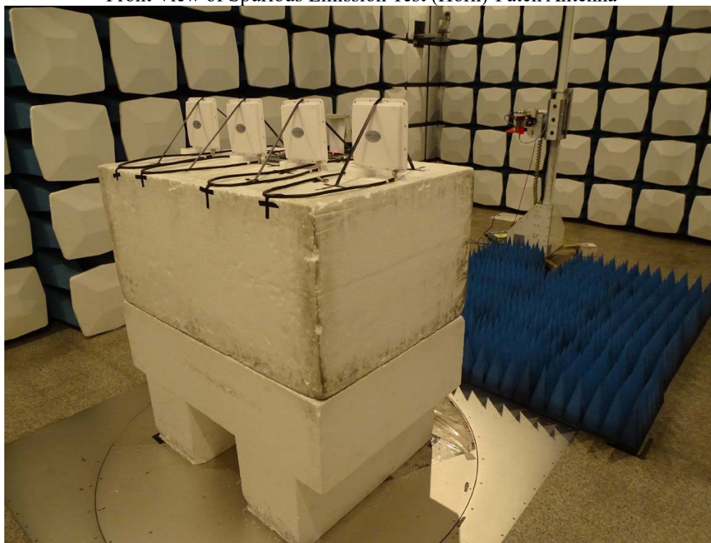
Front View of Spurious Emission Test (Horn)-Patch Antenna
