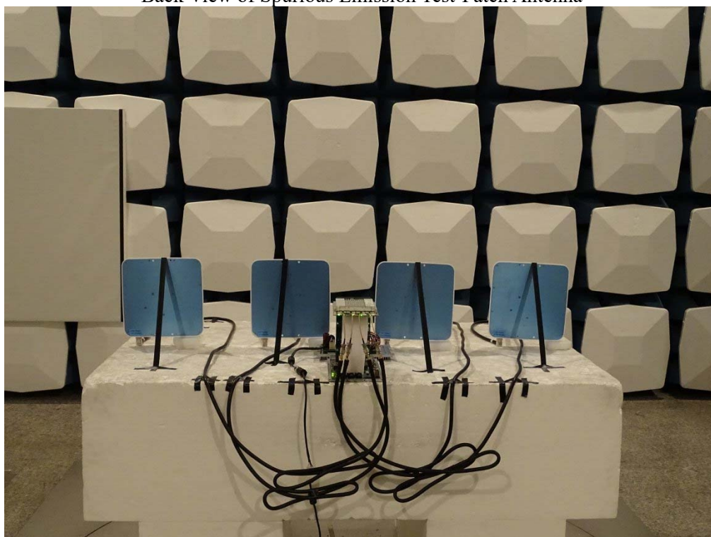
Back View of Spurious Emission Test-Patch Antenna
