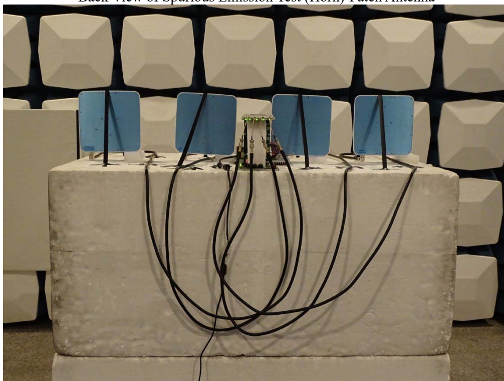
Back View of Spurious Emission Test (Horn)-Patch Antenna
