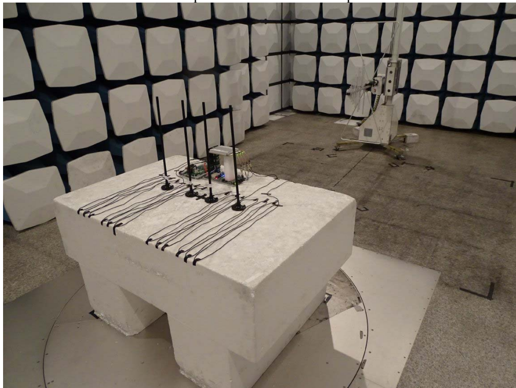
Front View of Spurious Emission Test-Dipole Antenna
