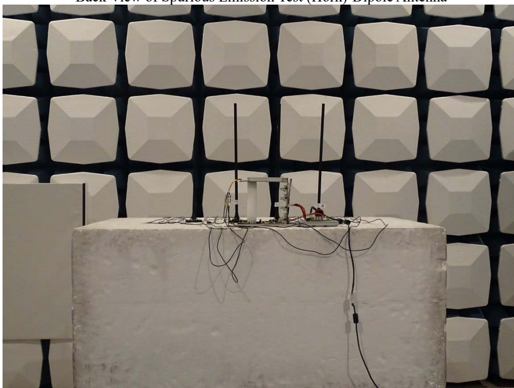
Back View of Spurious Emission Test (Horn)-Dipole Antenna
