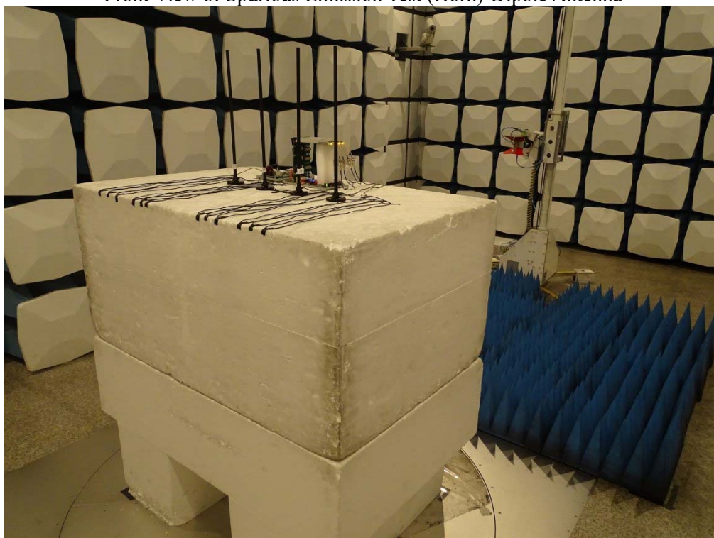
Front View of Spurious Emission Test (Horn)-Dipole Antenna
