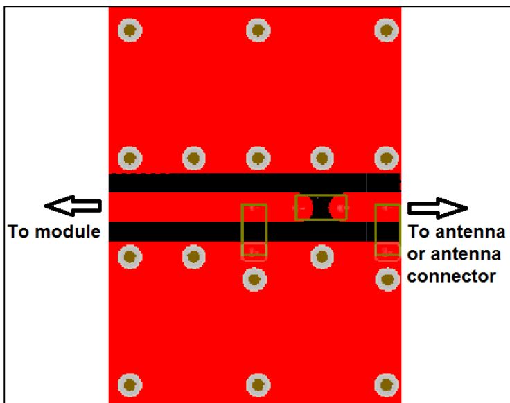
Figure 23. Controlled Impedance RF Trace Design
