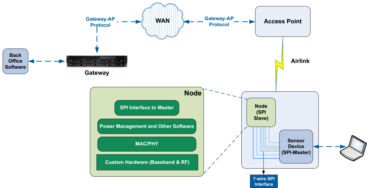
Figure 1. RPMA™ Network
