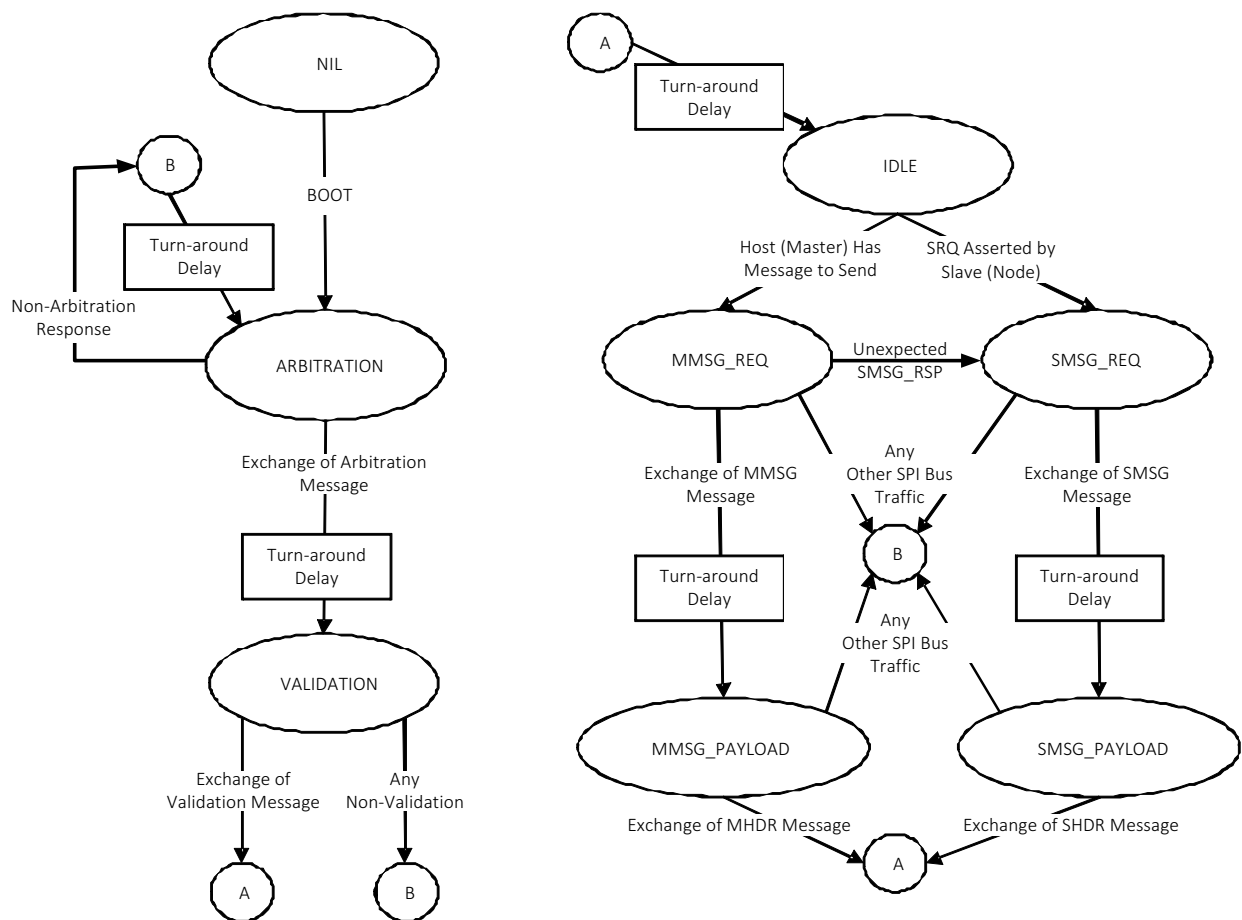
Figure 17. Host Interface SPI Bus State Machine
