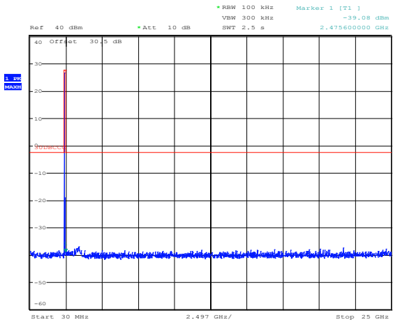
Figure 8.4-1: Conducted spurious emissions low channel
