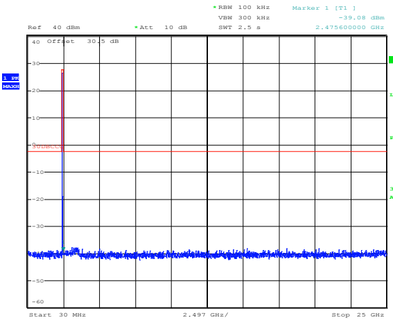
Figure 8.4-2: Conducted spurious emissions for high channel
