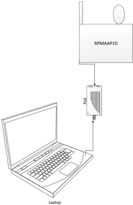
Figure 3.6-1: Setup diagram
