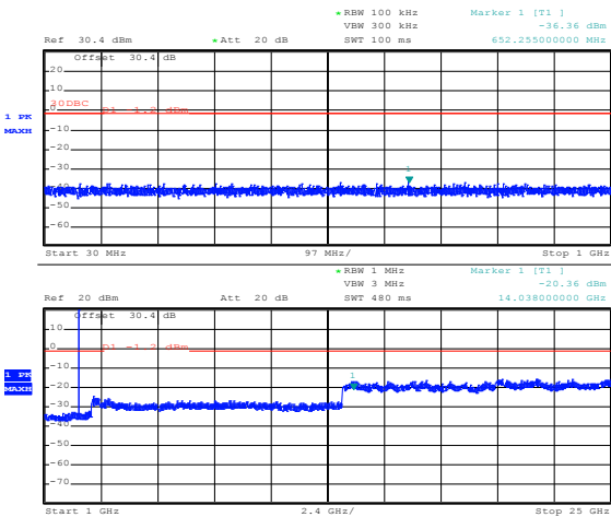
Figure 8.4-5: Conducted spurious emissions 2405.98 MHz
