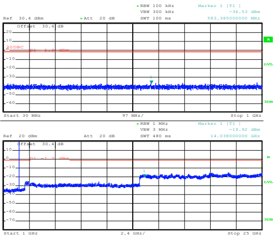
Figure 8.4-6: Conducted spurious emissions 2471.65 MHz
