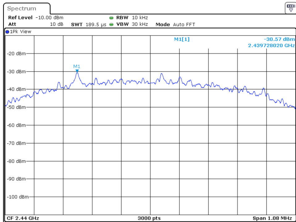
PSD – 2440 MHz
