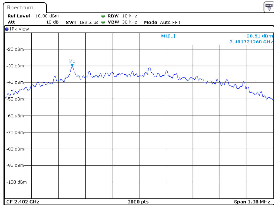
PSD – 2402 MHz
