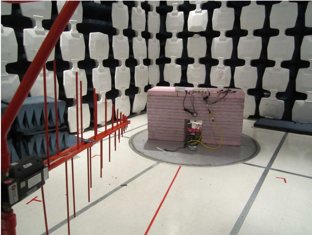
Radiated Emissions – 30 to 1000 MHz at 3m
