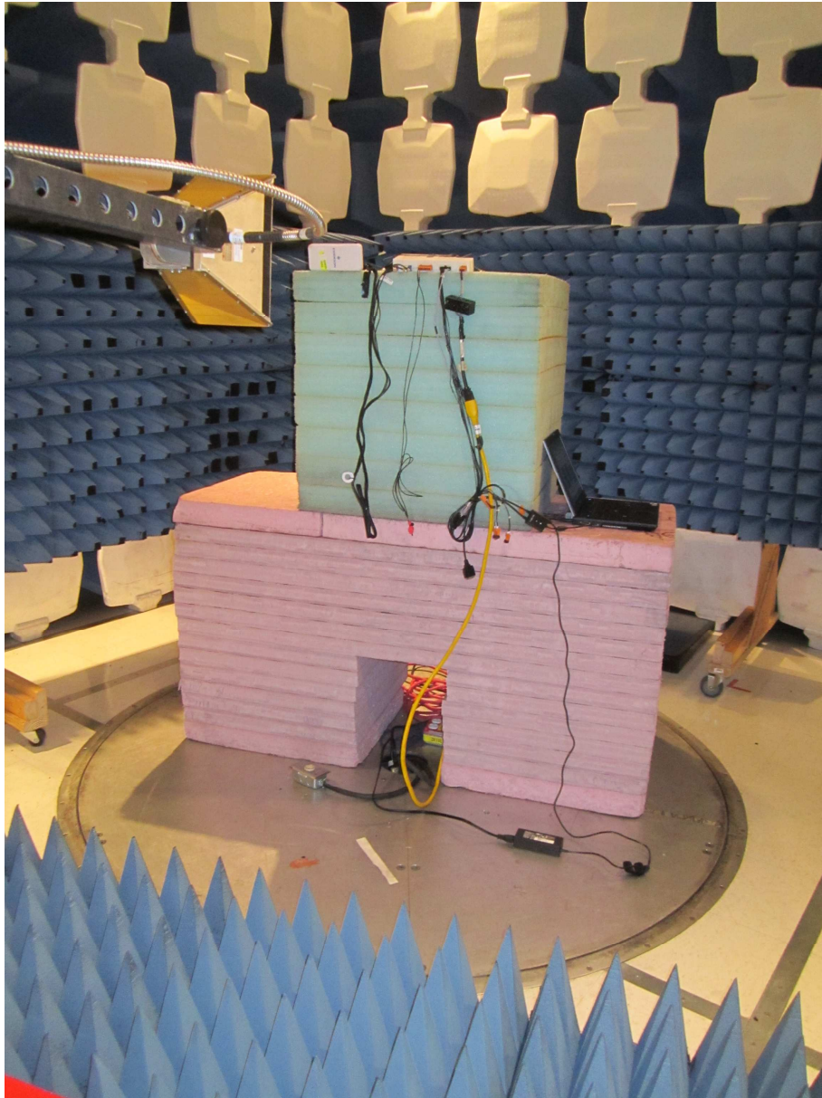
Radiated Emissions – 6 to 18 GHz at 1m
