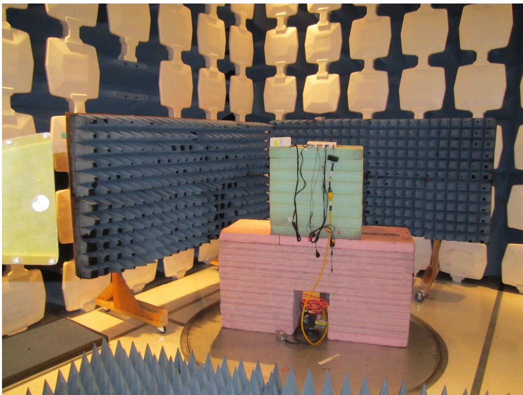
Radiated Emissions – 1 to 6 GHz at 3m
