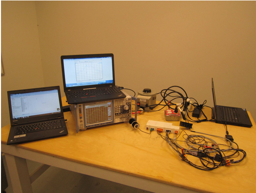
Conducted Measurements at the Antenna Port
