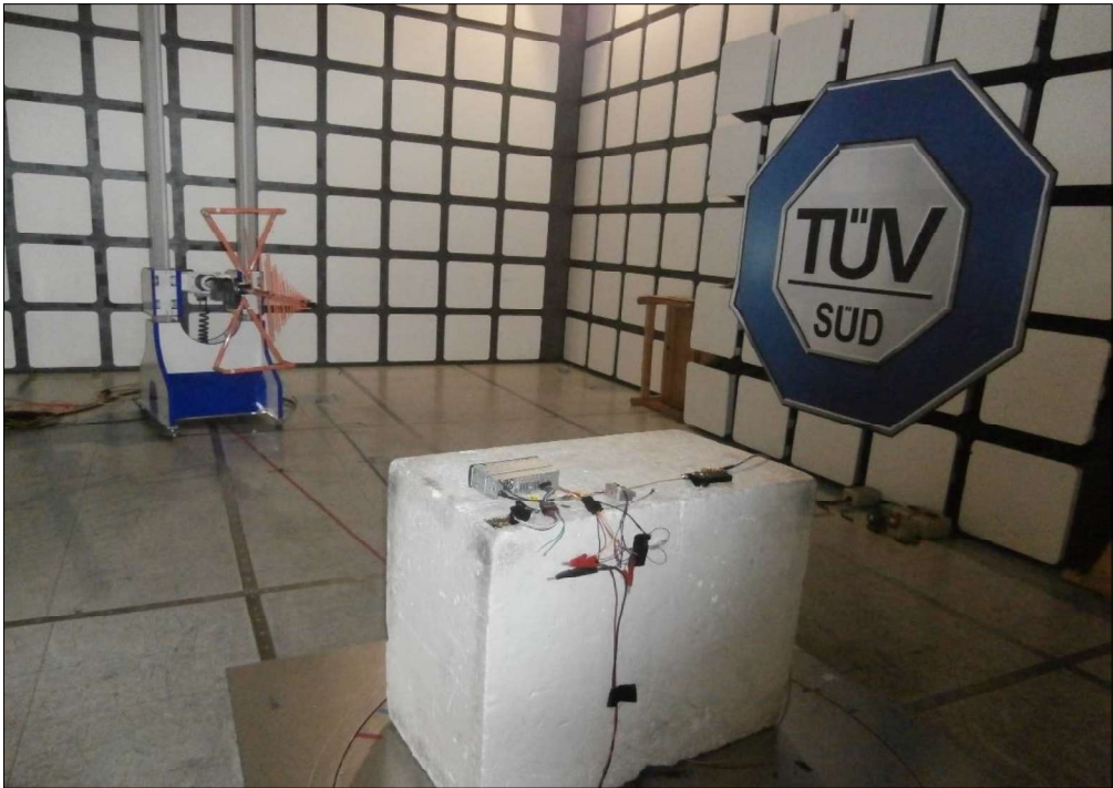
Figure 22 - Test Setup - Below 1 GHz
