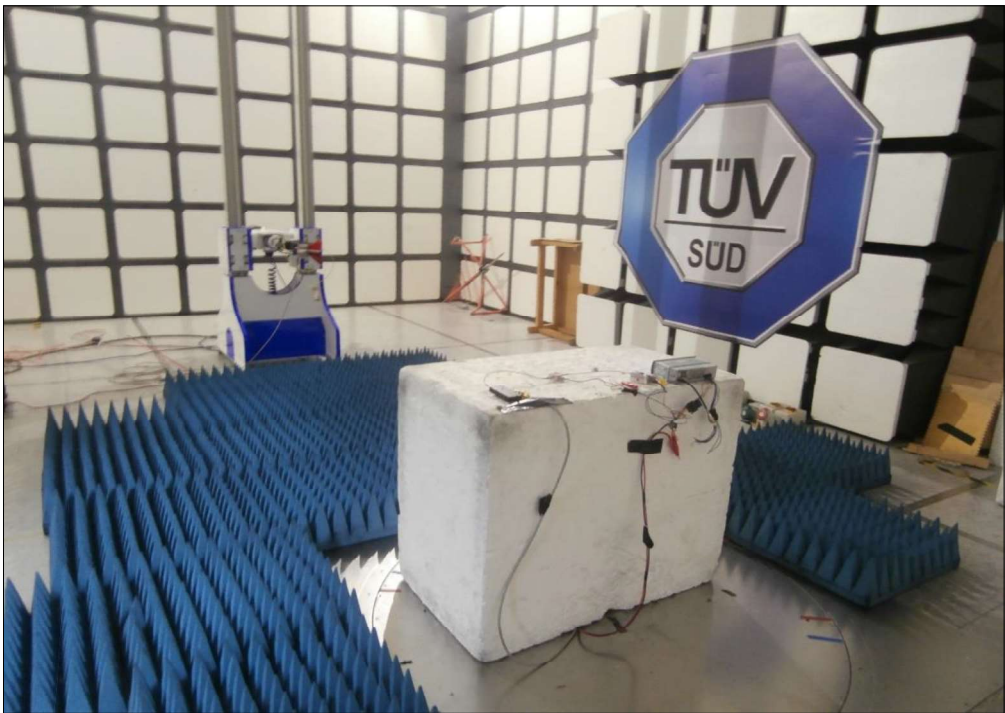
Figure 23 - Test Setup - Above 1 GHz
