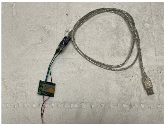
Figure 1.4.1-3– EUT with programming cable
