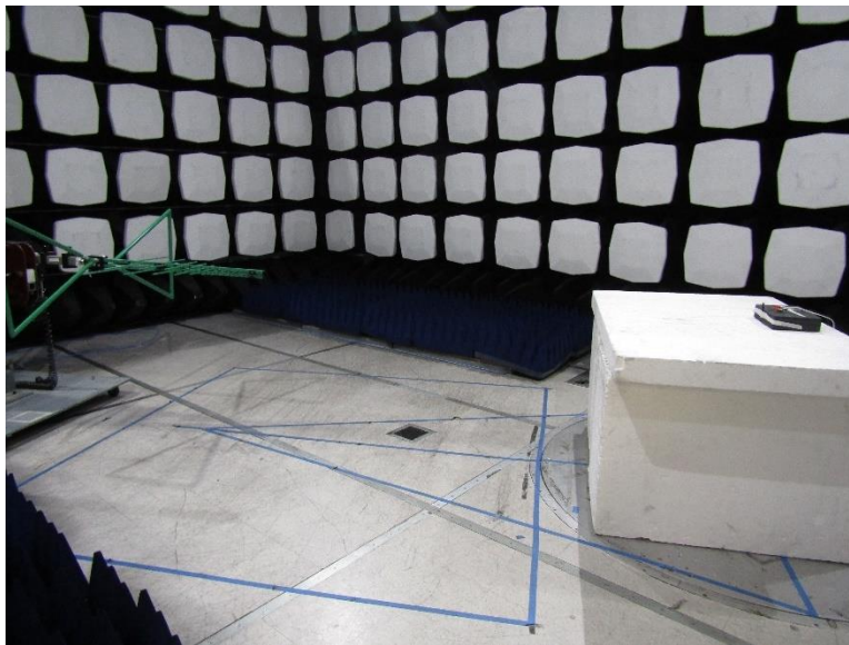
Figure-2 – Test Set up - Radiated Emissions <1 GHz
