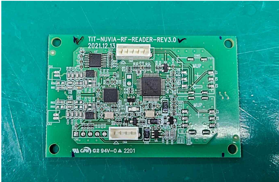
Card RFID board & Antenna
