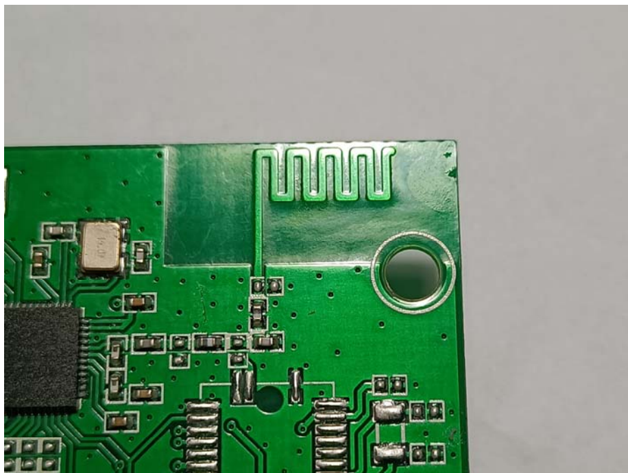
Closer View of Antenna
