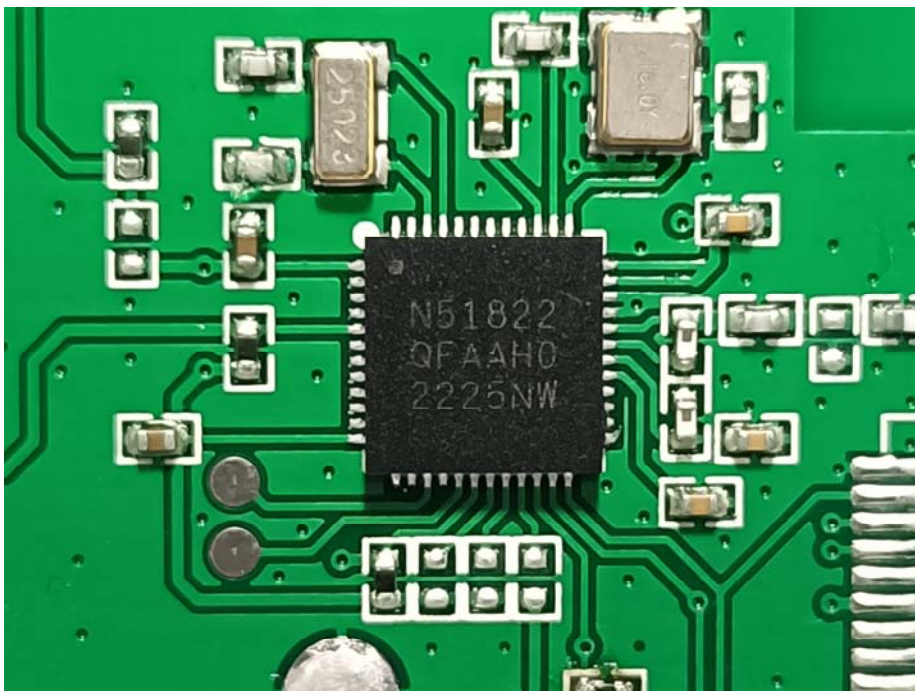
Closer View of IC
