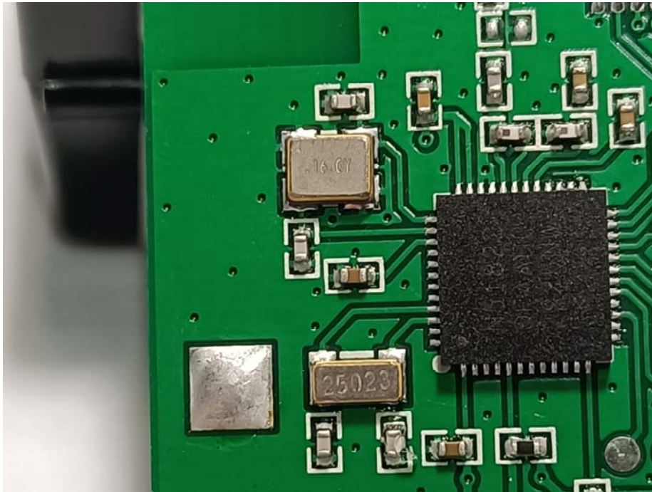
Closer View of Crystals
