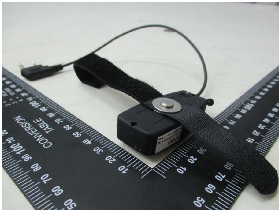
View of the EUT 8
