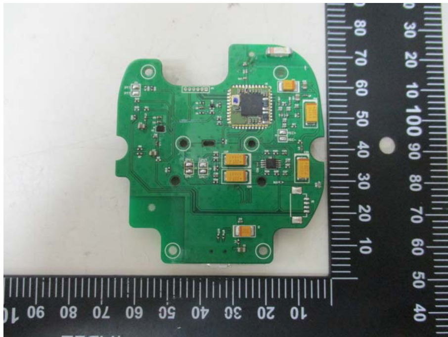
Front View of the PCB w/o metallic cover
