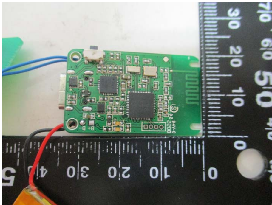
Rear View of PCB-1
