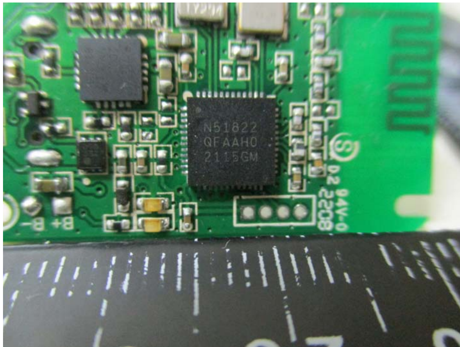
Closer View of BT module
