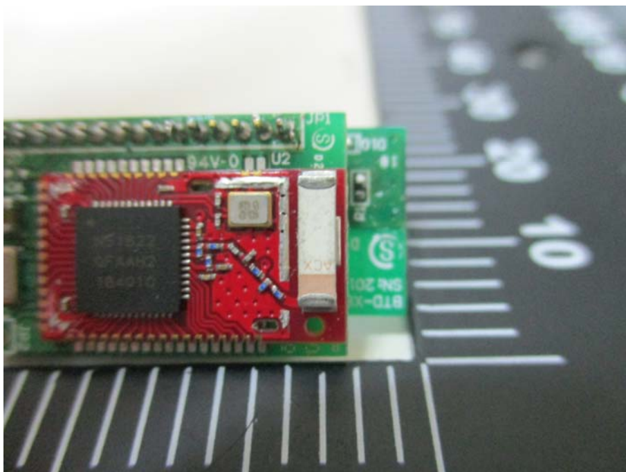
Close Up View of the Chip Antenna
