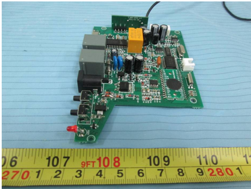
EUT –Rearboard Bottom View
