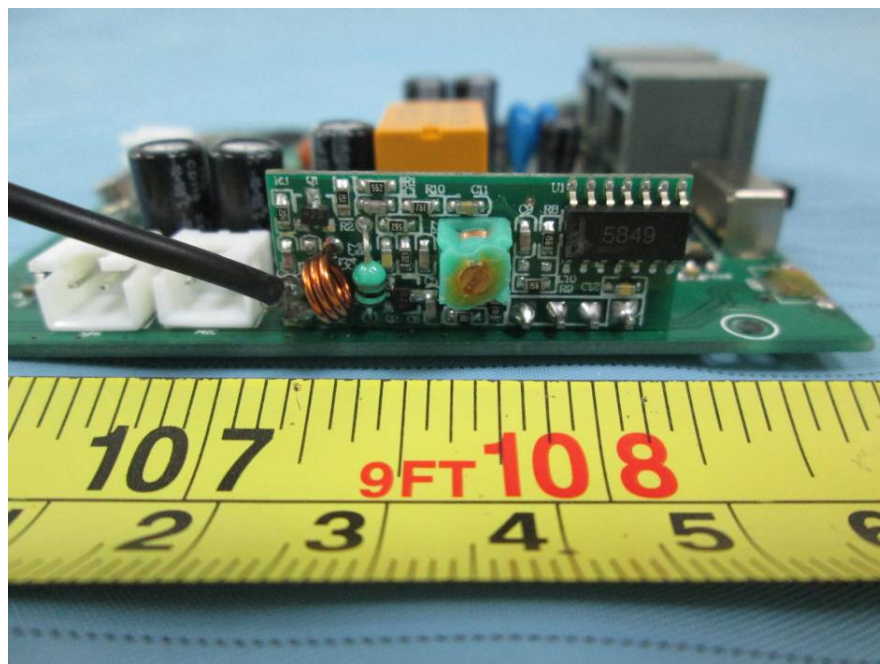
EUT –Rearboard Top View
