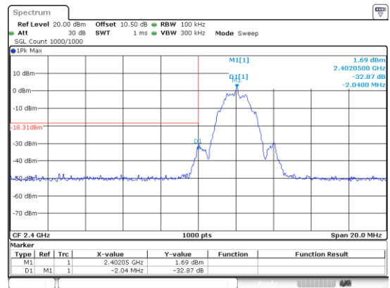
BLE_2M_Low_Channel
