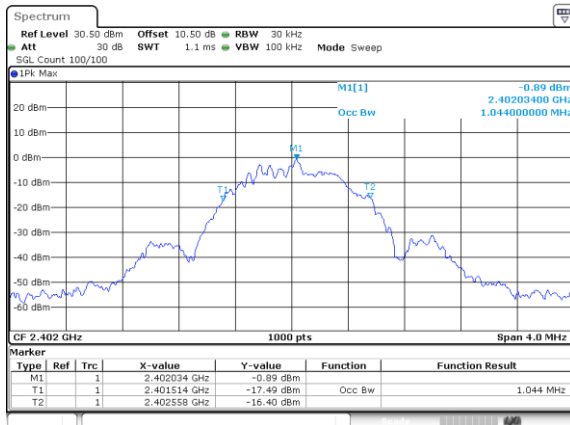
BLE_1M_Low_Channel
