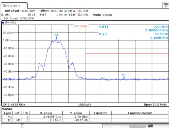
BLE_2M_High_Channel
