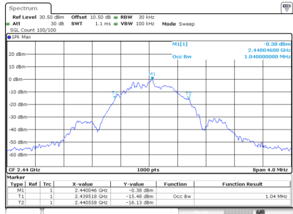
BLE_1M_Middle_Channel
