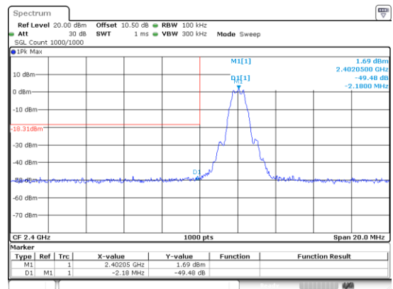
BLE_1M_Low_Channel
