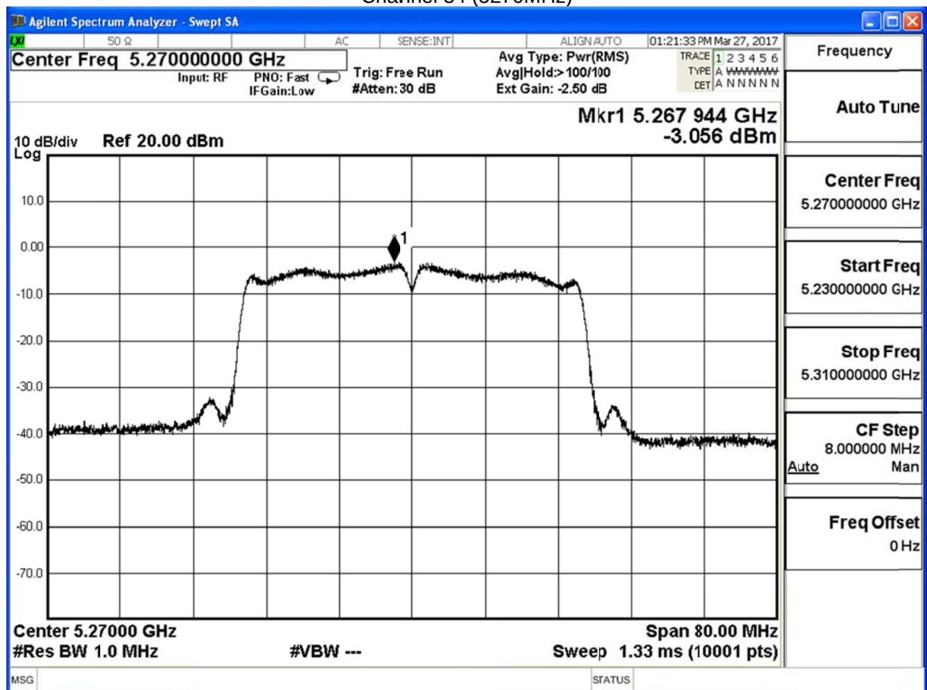
Channel 54 (5270MHz)
