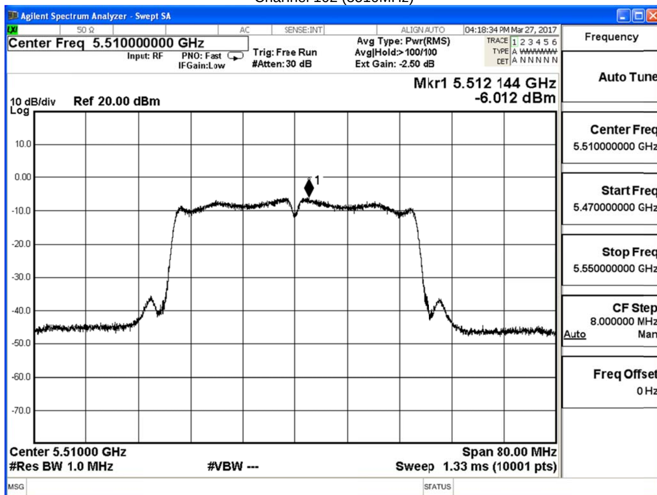
Channel 102 (5510MHz)
