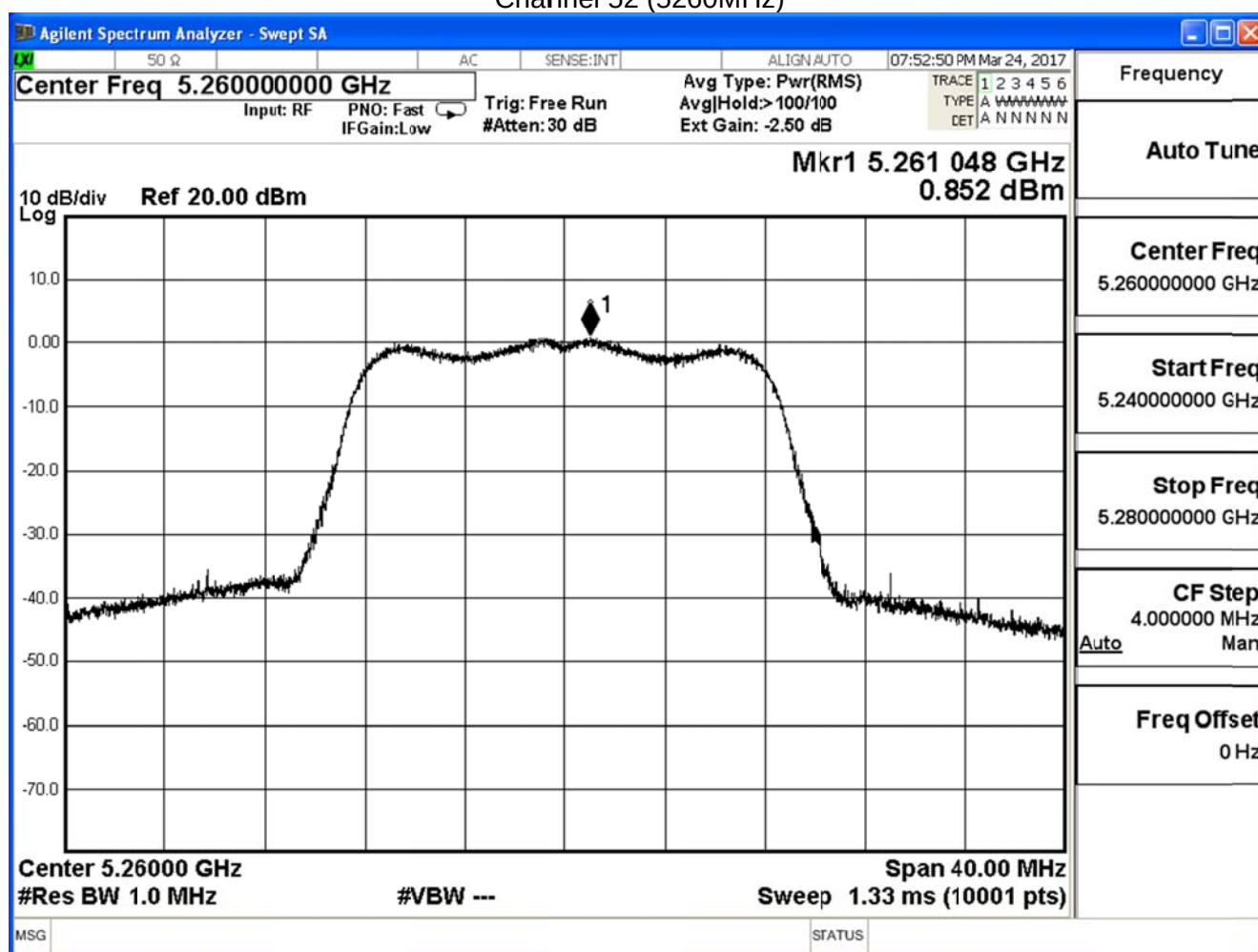
Channel 52 (5260MHz)
